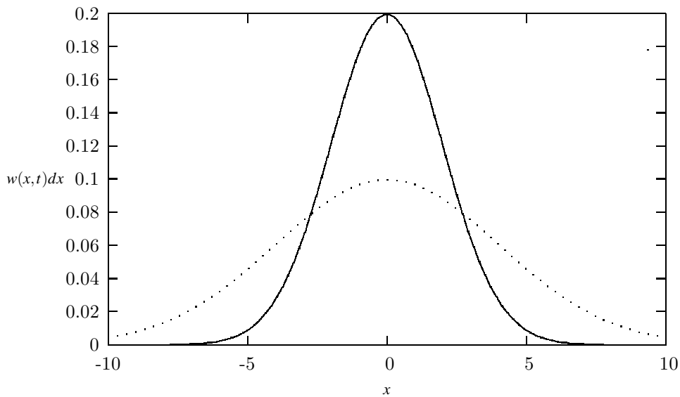
Fig. 12.1 Time development of a normal distribution with variance \sigma^2 = 2Dt and with D = 1\text{m}^2/\text{s} . The solid line represents the distribution at t = 2\text{s} while the dotted line stands for t = 8\text{s} .
