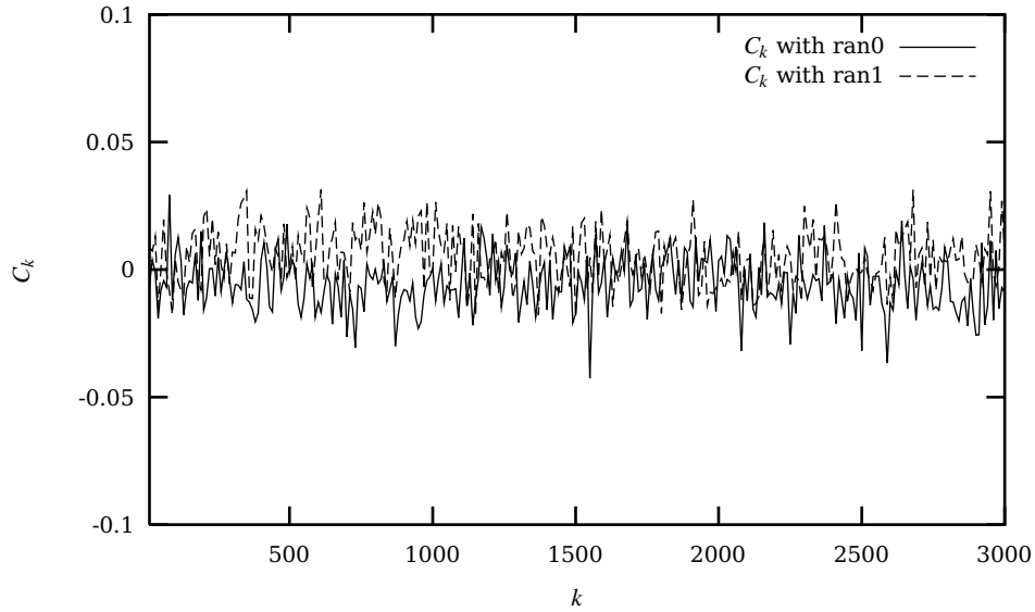
Fig. 11.3 Plot of the auto-correlation function C_k for various k -values for N = 10000 using the random number generators ran0 and ran1 .
