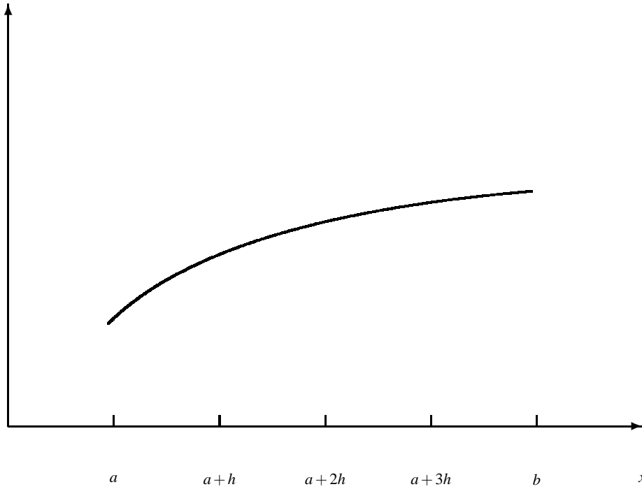
Fig. 5.1 The area encribed by the function f(x) starting from x = a to x = b . It is subdivided in several smaller areas whose evaluation is to be approximated by the techniques discussed in the text. The areas under the curve can for example be approximated by rectangular boxes or trapezoids.
