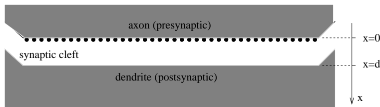
Fig. 10.7 Schematic drawing of the synaptic cleft in our model. The black dots represent neurotransmitter molecules, and the situation shown corresponds to the situation immediately after neurotransmitter release into the synaptic cleft.
