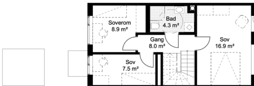
Plan 2 49 m²
