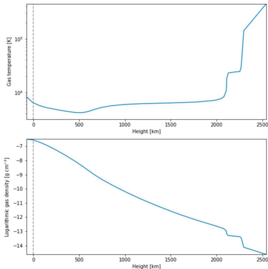
Fig. 1. The plot shows the semi-empirical atmosphere model C by Vernazza et al. (1981). Top: Gas temperature as function of height. Bottom: Logarithmic gas density as function of height. The vertical dashed line marks the height at which the optical depth \tau_{500\text{nm}} is unity, marking the bottom of the photosphere.
