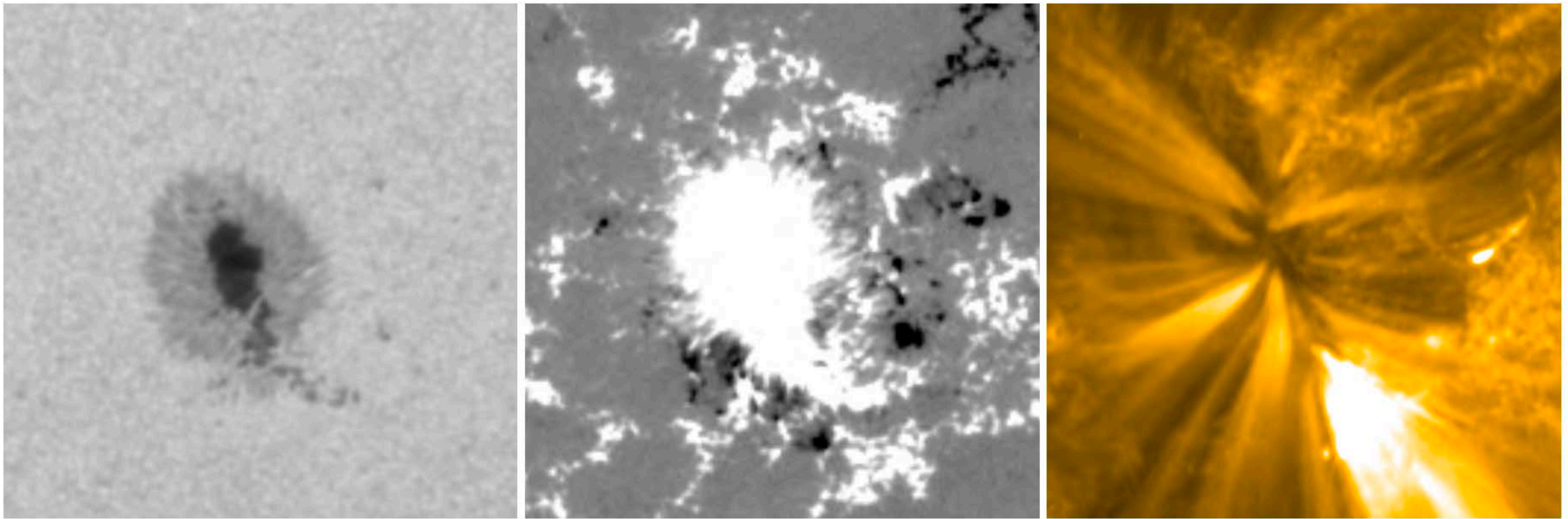
Fig. 2. In these three images we can see a sunspot observed with SDO at coordinates [x, y] = [+180'', -480''] on January 10 2022 at 08:57 UTC. The first image shows the HMI continuum, the second image shows the HMI magnetogram and the third image shows AIA 171.
