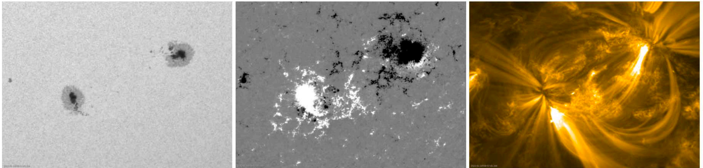
Fig. 2. The target sunspot at [x, y] = [+180'', -480''] is here the leftmost in the above images, with the rightmost being included just to show their different polarities. In the magnetogram we clearly see that the two sunspots have opposite polarities, and we therefore expect magnetic field lines to connect these two regions. This is observed in the third image, where we clearly see that plasma has oriented itself with the magnetic field lines, clearly connecting the two sunspots.
