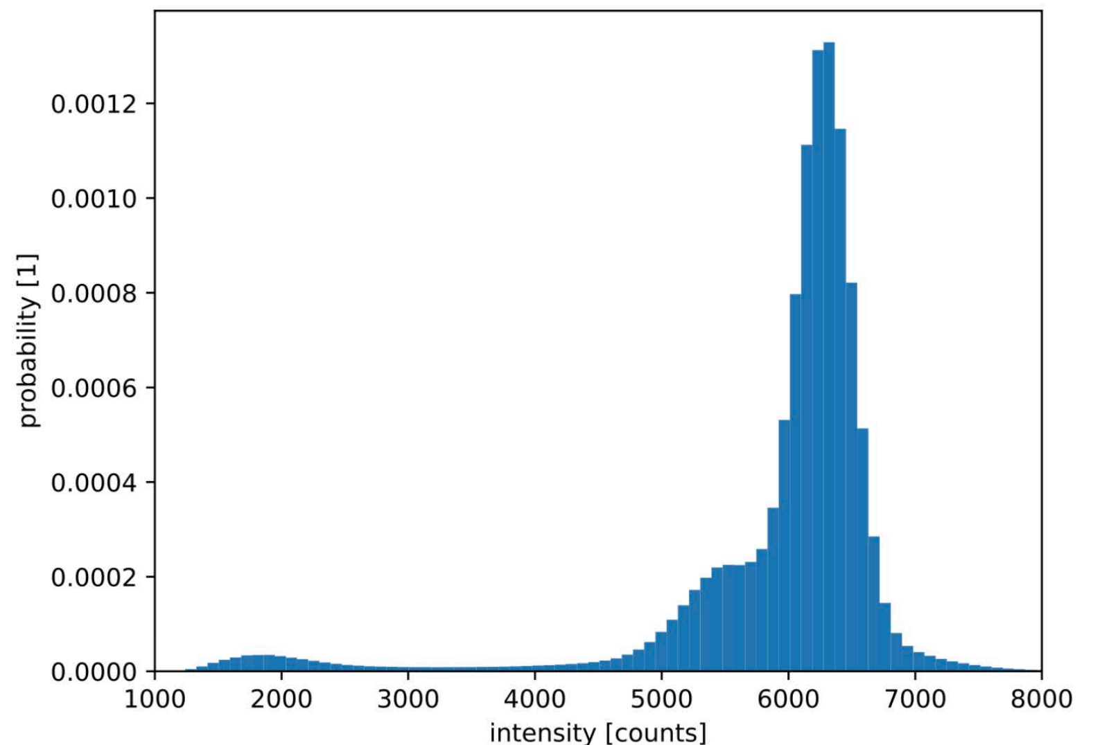
Fig. 4. Histogram of the intensity values of the shortest wavelength in the data set obssun_sst3/obssun_sst3.h5 , over all time steps.
