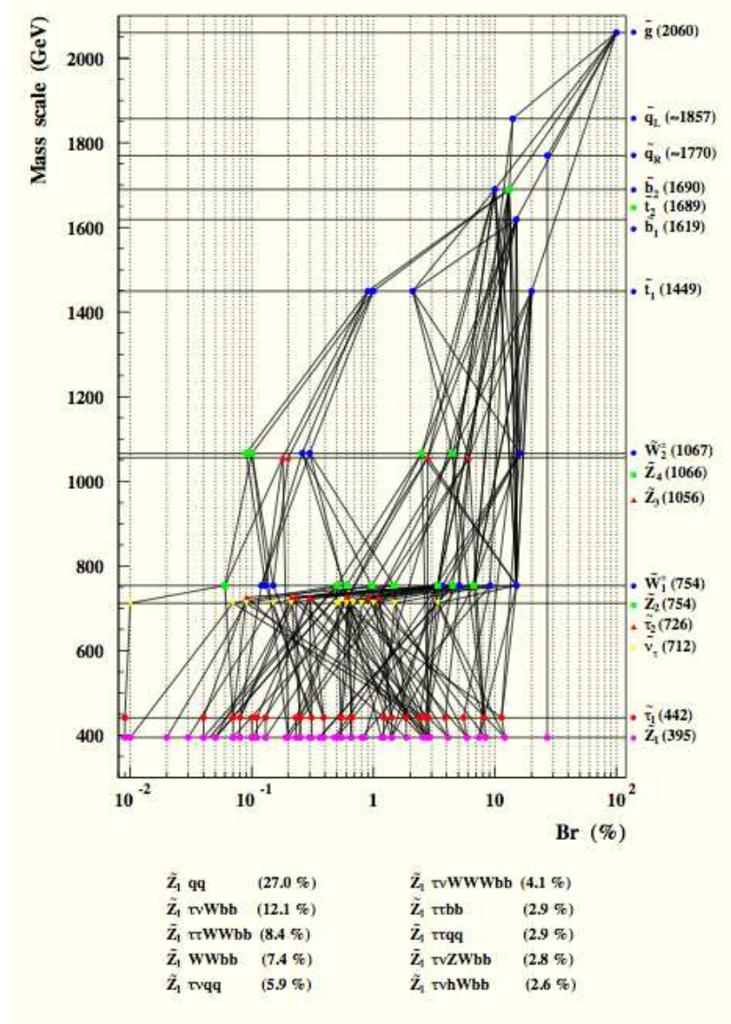
Figure 6.2: Possible cascades for an MSSM model with a 2060 GeV gluino as the heaviest sparticle.
