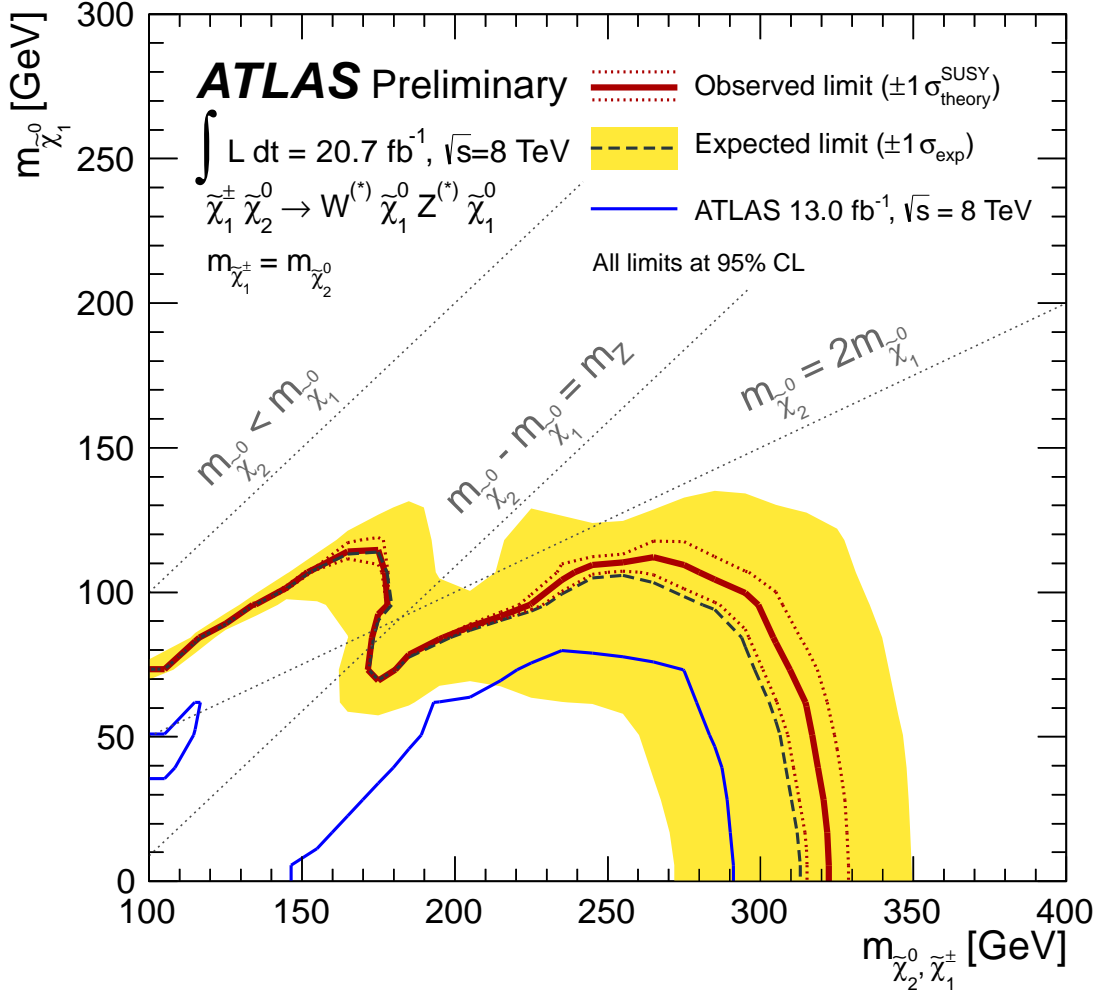
Figure 6.15: Plot of the excluded area in the (m_{\tilde{\chi}_1^\pm}, m_{\tilde{\chi}_1^0}) plane assuming m_{\tilde{\chi}_1^\pm} = m_{\tilde{\chi}_2^0} [20].
