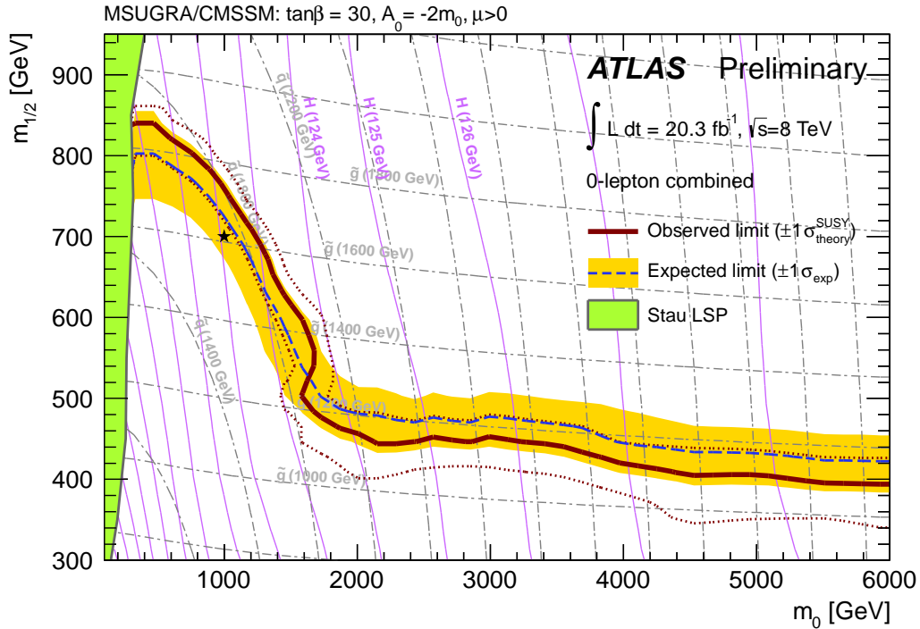
Figure 6.10: Plot of the excluded area in the m_{1/2} - m_0 plane of the mSUGRA parameter space for \tan\beta = 30 , A_0 = -2m_0 and \mu > 0 . The limit is the red line. The green area is theoretically forbidden because it has a charged LSP (the stau) [17].
