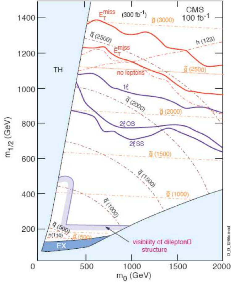
Figure 6.5: Plot of the projected discovery reach for different values of common GUT scale gaugino mass m_{1/2} and scalar mass m_0 at 100 \text{ fb}^{-1} at the Compact Muon Spectrometer (CMS). The light blue area represents theoretical limits. The dark blue area is the parameter space probed by the Tevatron. The lower red line represents a pure \cancel{E}_T search at 14 TeV, the upper red line represents the same search with three times the statistical data. The blue lines represent searches using leptons. The dotted lines show the masses of different particles.
