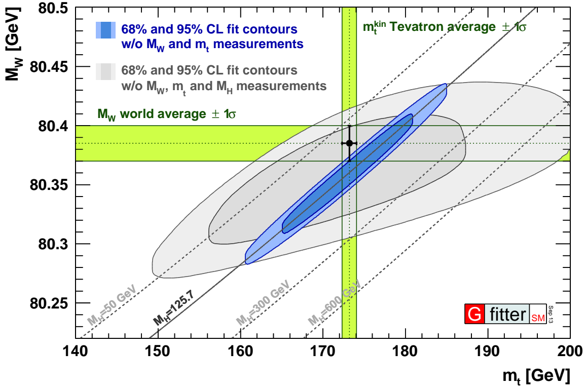
Figure 6.22: Electroweak fit excluding M_W and m_t (blue), compared to their measured values (green) [21].
