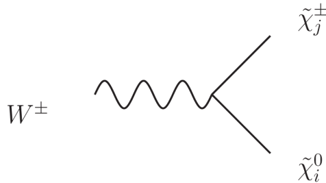
Figure 6.17: Coupling W - \tilde{\chi}_i^0 - \tilde{\chi}_j^\pm .
