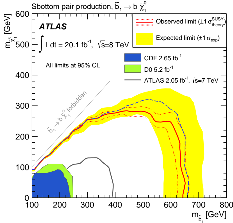
Figure 6.11: Plot of the excluded area in the (m_{\tilde{b}_1}, m_{\tilde{\chi}_1^0}) plane. The limit from ATLAS is the red line, while the green and blue colored areas are excluded from different Tevatron experiments [18].
