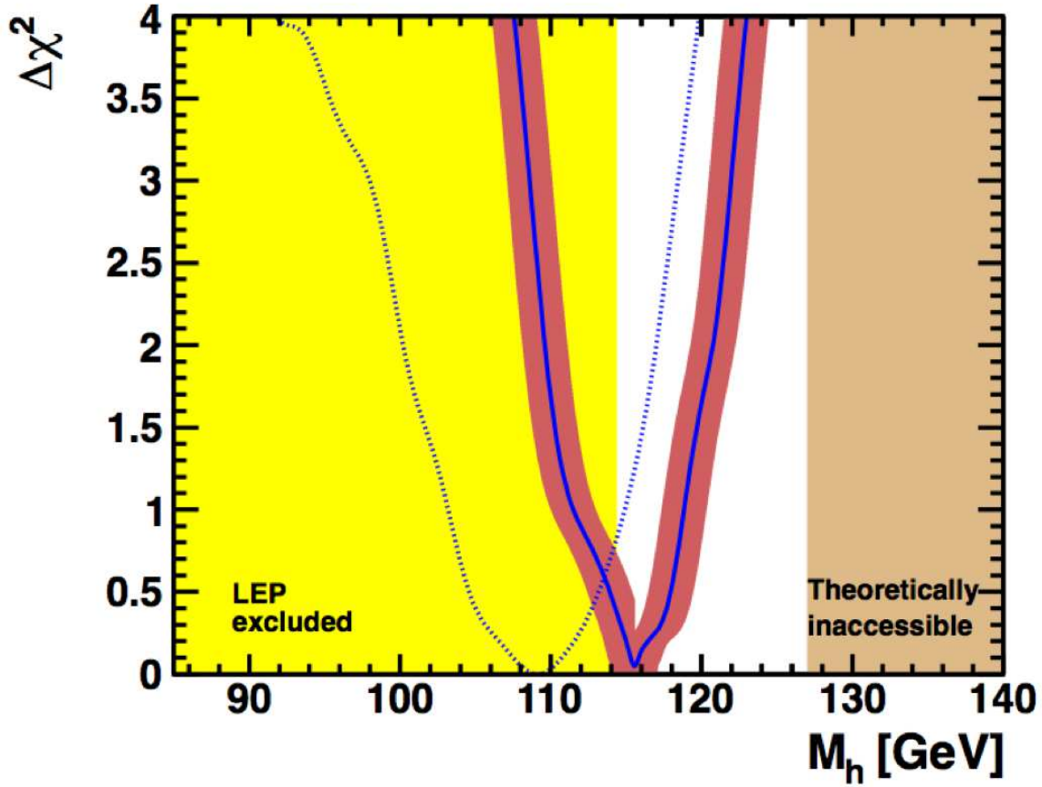
Figure 6.21: Plot of the \Delta\chi^2 from all precision variable measurements for mSUGRA as a function of the Higgs mass. The yellow area shows the experimentally excluded area, while the brown shows the theoretically inaccessible area.
