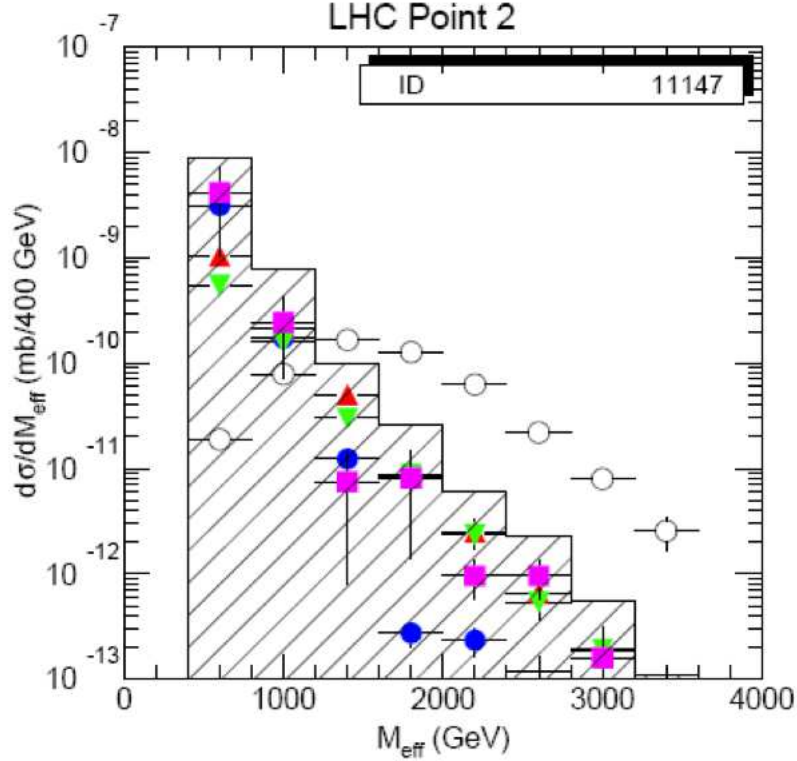
Figure 6.4: Plot of the differential cross section with respect to effective mass, plotted against the effective mass of the final state particles as given in (6.1). The colored data points represent different SM processes, and the histogram is the sum of all SM contributions, while the white circles represent a possible supersymmetry scenario. The position of the supersymmetry signal maximum is correlated to the masses of \tilde{\chi} and \tilde{q} , but there is large variance.
