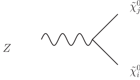
Figure 6.18: Coupling Z - \tilde{\chi}_i^0 - \tilde{\chi}_j^0 .
