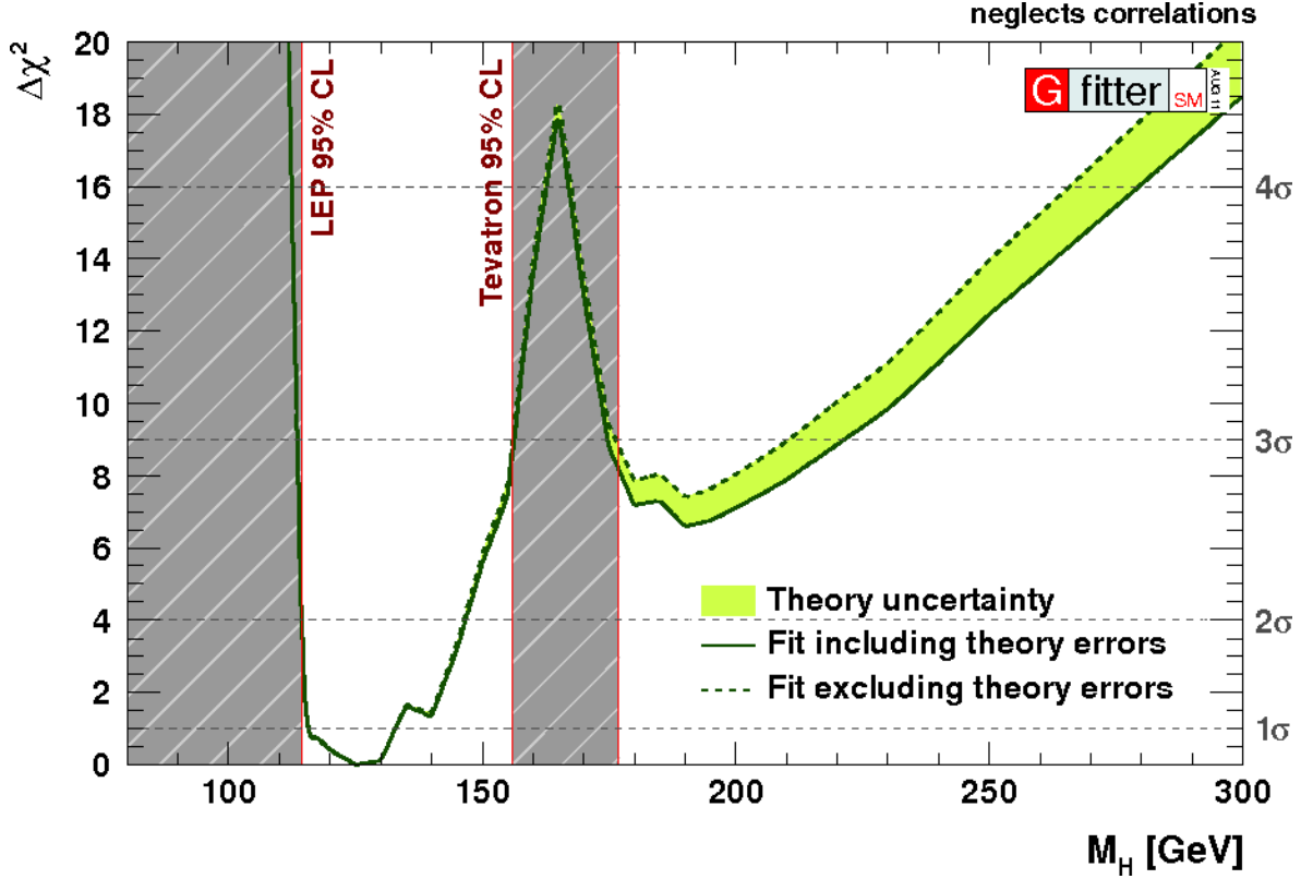
Figure 6.20: Plot of the total \Delta\chi^2 from all precision variable measurements and the direct exclusions bounds for the SM Higgs from LEP and the Tevatron, as a function of the Higgs mass.
