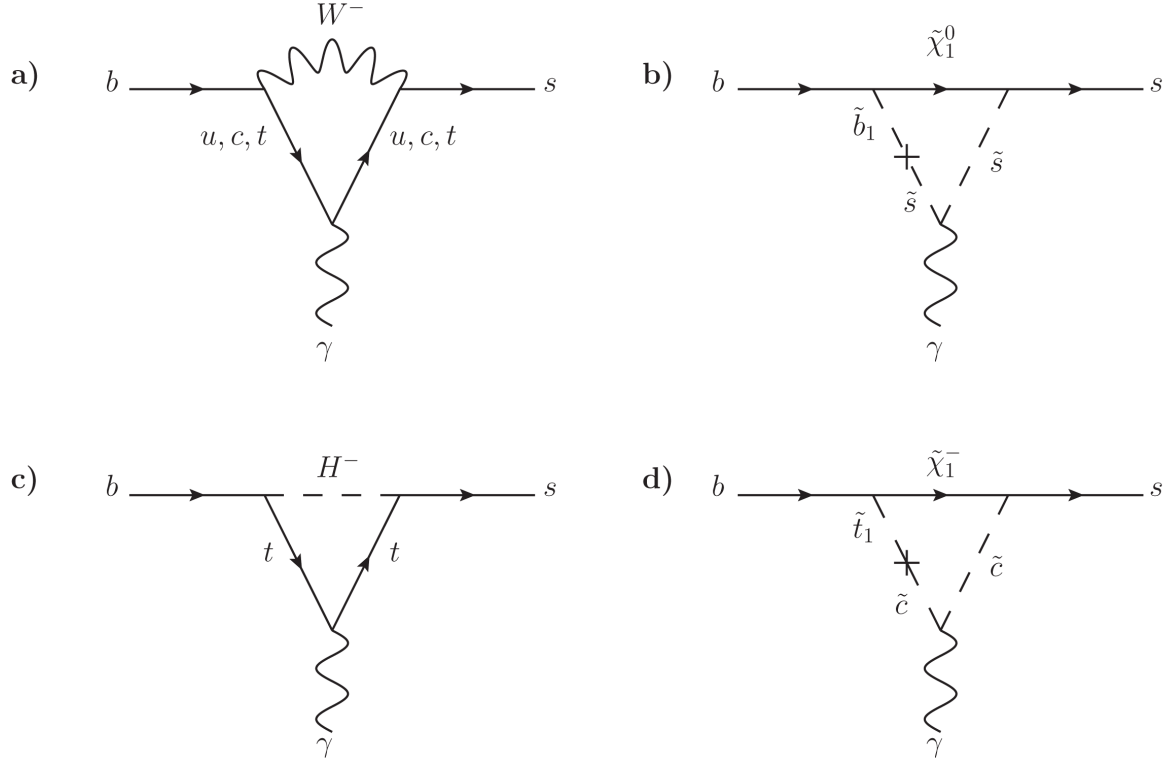
Figure 6.24: Diagrams for the process b \rightarrow s\gamma . a) shows the SM diagram while b), c) and d) show MSSM contributions.
