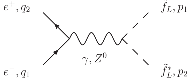
Figure 6.16: Feynman diagram for the pair production of left-handed sfermions in the s-channel at a linear collider.
