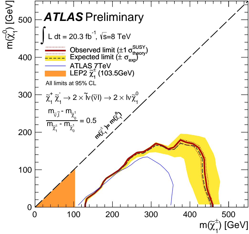
Figure 6.14: Plot of the excluded area in the (m_{\tilde{\chi}_1^\pm}, m_{\tilde{\chi}_1^0}) plane [19].
