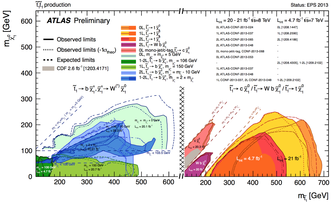
Figure 6.12: Plot of the excluded area in the (m_{\tilde{t}_1}, m_{\tilde{\chi}_1^0}) plane for the two main decay categories. References for the individual analysis given in figure.
