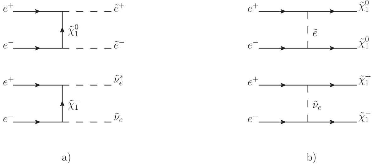
Figure 6.19: The t-channel diagrams for pair production of selectrons and electron sneutrinos a) and gauginos b).
