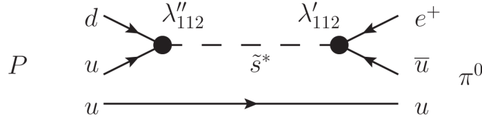
Figure 5.2: Feynman diagram for proton decay with RPV couplings.
