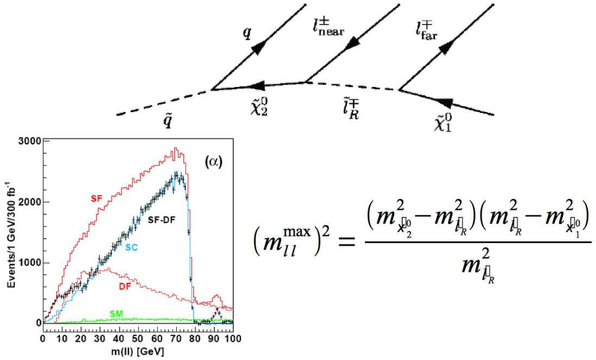
Figure 6.6: To measure the masses of supersymmetric particles for a given decay chain with three sequential two-body decays we can take the invariant mass between two particles, say the two leptons, plot it and find the endpoint. This gives us one relationship between the masses (displayed above). We then do the same thing with the other two possible combinations in order to get three equations with three unknowns.
