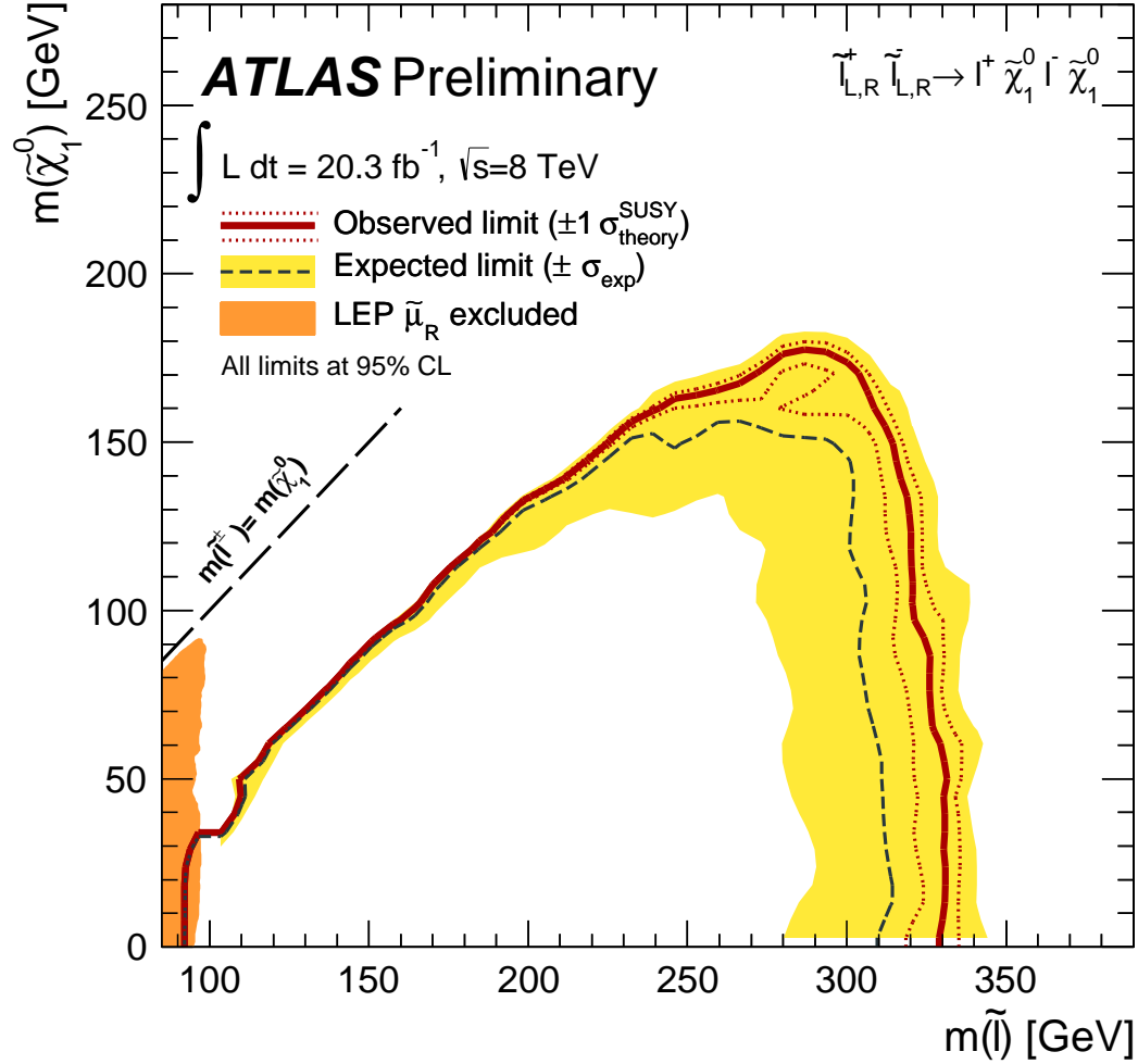
Figure 6.13: Plot of the excluded area in the (m_{\tilde{l}}, m_{\tilde{\chi}_1^0}) plane for mass degenerate right- and left-handed smuons and selectrons [19].
