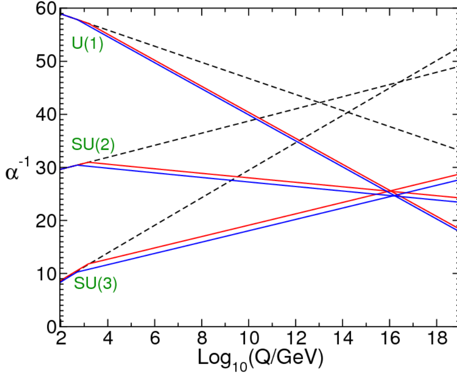
Figure 5.5: RGE evolution of the inverse gauge couplings \alpha_i^{-1}(Q) in the SM (dashed lines) and the MSSM (solid lines). In the MSSM case, the sparticle mass thresholds are varied between 250 GeV and 1 TeV and \alpha_3(m_Z) between 0.113 and 0.123 to create the bands shown by the red and blue lines. Two-loop effects are included.
