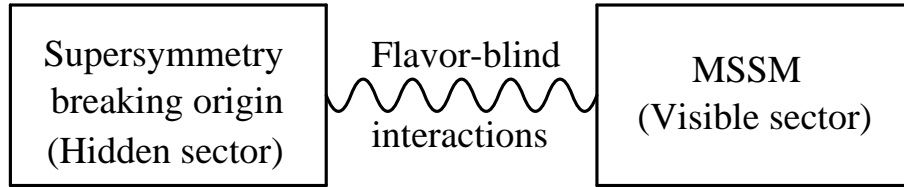
Figure 6.7: A generic illustration of how to generate soft breaking terms [16].
