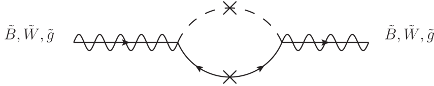
Figure 6.9: Diagram for GMSB. The messenger scalars and fermions run in the loop.
