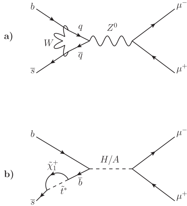
Figure 6.25: Diagrams for the process B_s \rightarrow \mu^+ \mu^- . Diagram a) shows the leading SM contributions, while b) shows one contribution from the MSSM.
