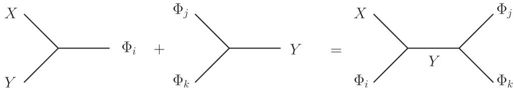
Figure 6.8: Interactions leading to effective 4-particle couplings in our example.
