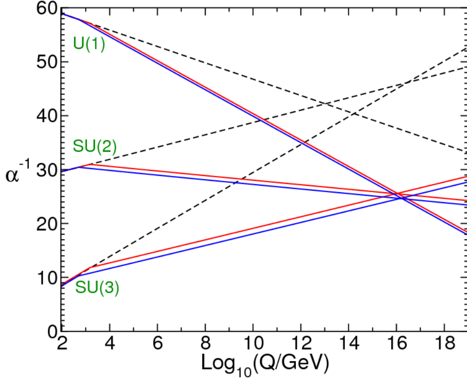
Figure 7.3: The RGE evolution of the inverse gauge couplings \alpha_i^{-1}(Q) in the Standard Model (dashed lines) and the MSSM (solid lines). In the MSSM case, the sparticle mass thresholds are varied between 250 GeV and 1 TeV and \alpha_3(m_Z) between 0.113 and 0.123 to create the bands shown by the red and blue lines. Two-loop effects are included.
