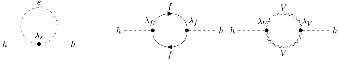
Figure 5.1: Higgs self-energy diagrams with scalars s (left), fermions f (middle), and vectors V (right). The dots indicate vertices with the given coupling strength.
