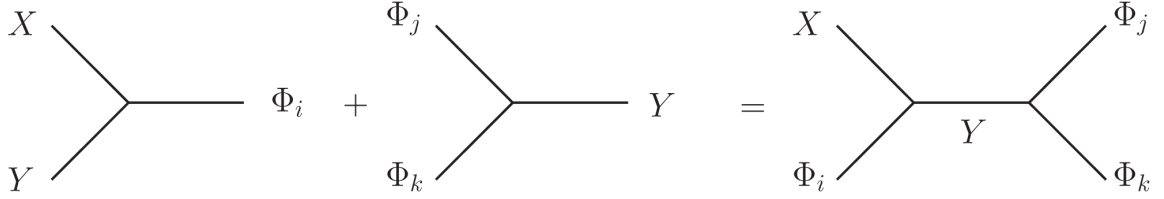
Figure 6.2: Interactions leading to effective 4-superfield couplings in our example. X is the scalar superfield which is breaking supersymmetry, while Y is the mediator superfield which transmits the effect of this breaking to the MSSM fields \Phi_i .
