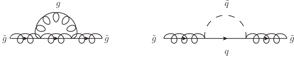
Figure 7.5: One loop contributions to the gluino mass.
