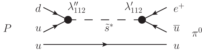
Figure 7.2: Possible Feynman diagram for proton decay with R-parity violating couplings \lambda''_{112} and \lambda'_{112} .
