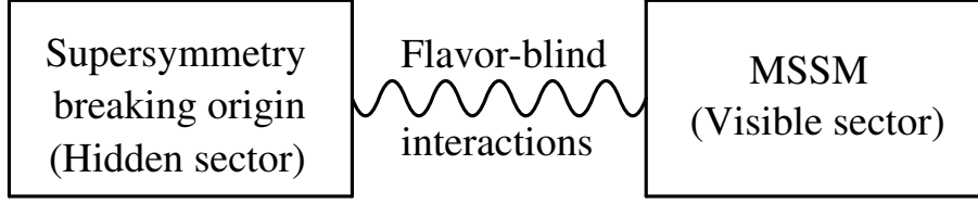
Figure 6.1: A generic illustration of how to generate soft breaking terms. Taken from Ref. [18].
