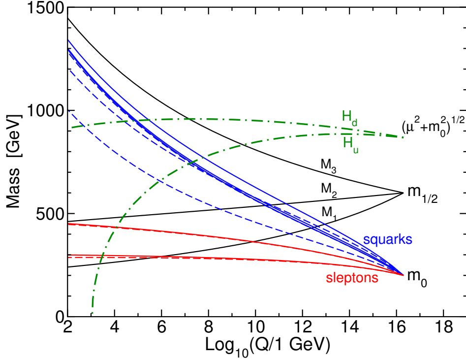
Figure 7.4: The RGE evolution of soft-mass parameters in the MSSM with typical minimal supergravity-inspired boundary conditions imposed at 2 \cdot 10^{16} GeV. The parameter values used for this illustration were m_0 = 200 GeV, m_{1/2} = -A_0 = 600 GeV, \tan \beta = 10 , and \text{sgn}(\mu) = + .
