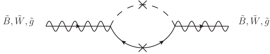
Figure 6.3: Diagram for GMSB giving masses to the gauginos \tilde{g} , \tilde{B} , and \tilde{W} , in the MSSM. The messenger scalars and fermions run in the loop.
