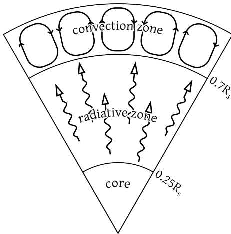
Figure 1: Sketch of the internal structure of the Sun.
