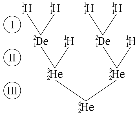
Figure 2: The ppI-chain.
