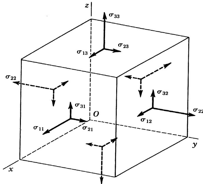
FIGURE 2-1. Stress distribution on an infinitesimal volume element.
