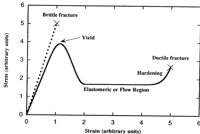
Figure 8.7. Illustrating brittle and ductile materials.
