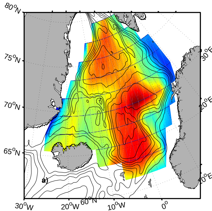
Figure 3.16: Geostrophic contours (solid lines) in the Nordic seas. Superimposed are contours showing the first EOF of sea surface height derived from satellite measurements. The latter shows strong variability localized in regions of closed q_s contours. From Isachsen et al. (2003).
