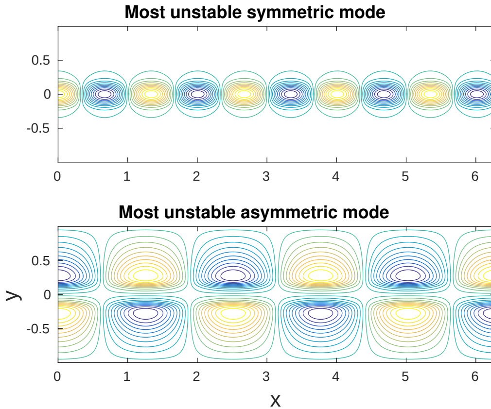
Figure 3.21: The most unstable symmetric and asymmetric waves for the eastward \text{sech}^2 jet.
