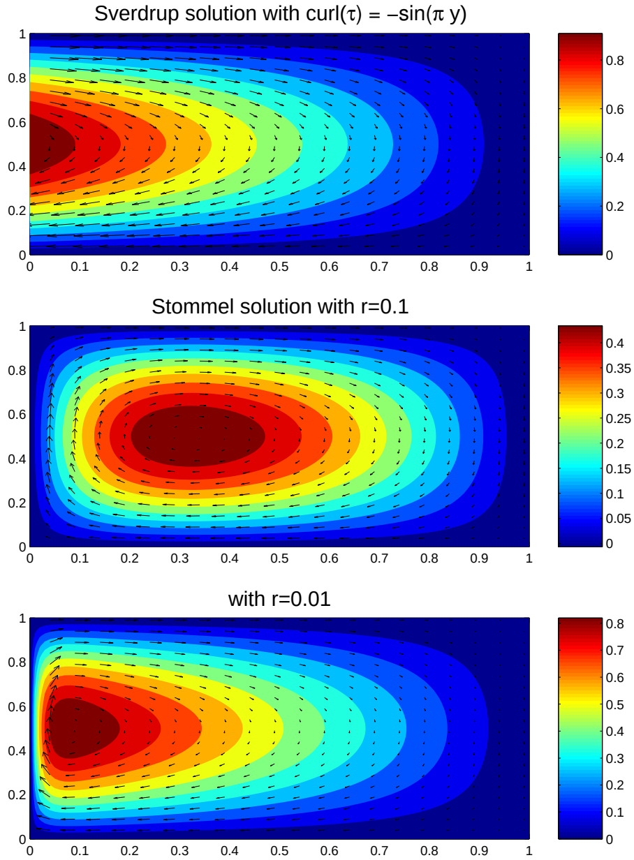
Figure 3.15: Solutions of Stommel's model for two different values of the friction coefficient, r .
