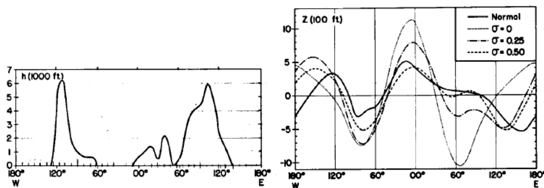
Figure 3.13: Charney and Eliassen's (1949) solution of the barotropic mountain wave problem at 45N. The topographic profile is shown in the left panel (their Fig. 3). The mean pressure at 500 mb is shown in the right panel (their Fig. 4) as the solid line. The dashed lines indicate the theoretical solutions, using three different values of friction.
