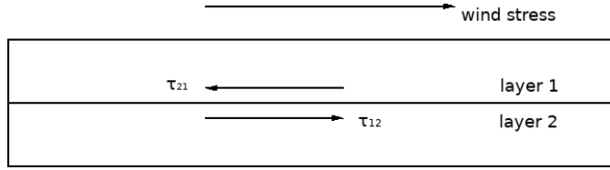
Figure 3.10: The wind acting on an upper layer of fluid at the surface. The layer exerts stress on the layer below, which produces an equal and opposite stress on the upper layer.
