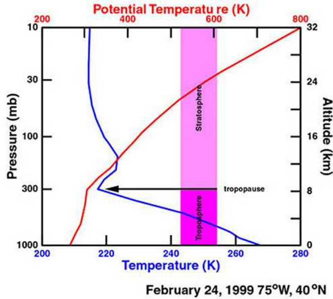
Figure 1.6: The potential temperature and temperature in the lower atmosphere. Courtesy of NASA/GSFC.
