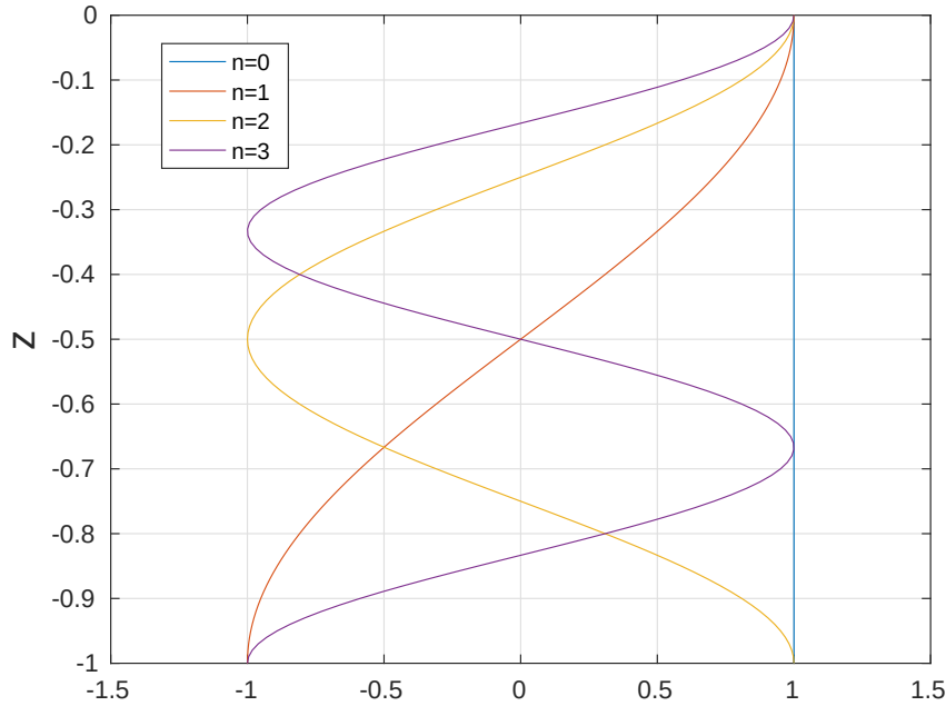
Figure 4.1: The baroclinic modes with constant stratification.
