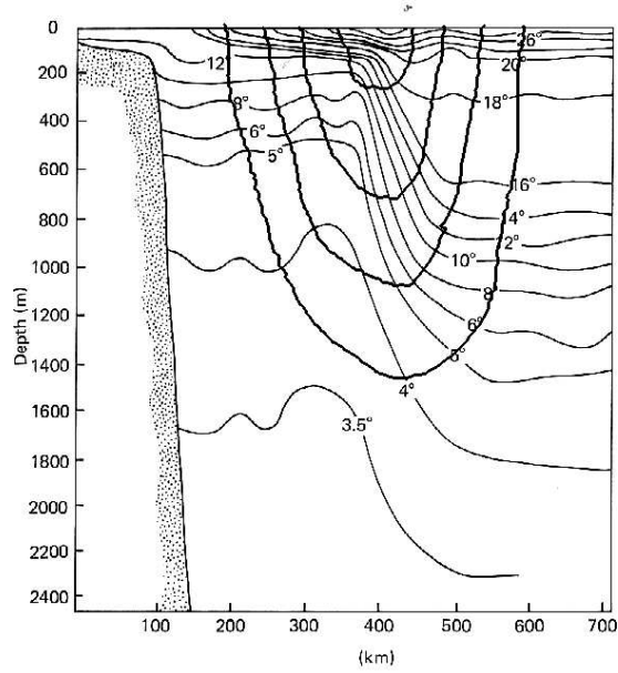
Figure 2.13: A cross section of the ocean temperature in the core of the Gulf Stream.
