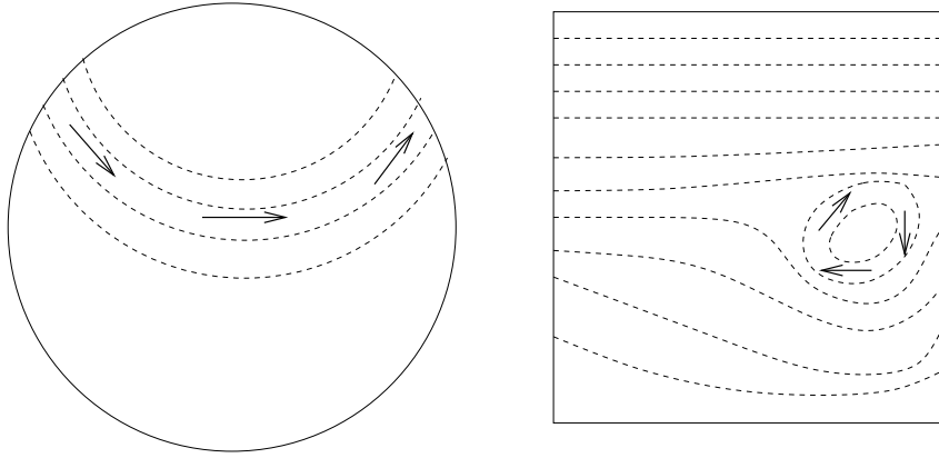
Figure 3.3: Steady, along-geostrophic contour flow in the atmosphere (left) and in the ocean (right).
