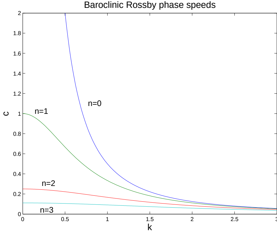
Figure 4.2: Rossby phase speeds as a function of wavenumber for the first four modes.
