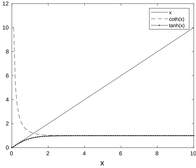
Figure 4.11: x , \tanh(x) and \coth(x) .
