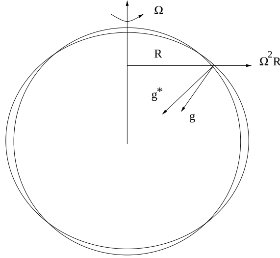
Figure 1.4: The centrifugal force and the deformed earth. Here g is the gravitational vector for a spherical earth, and g^* is that for the actual earth. The latter is an oblate spheroid .
