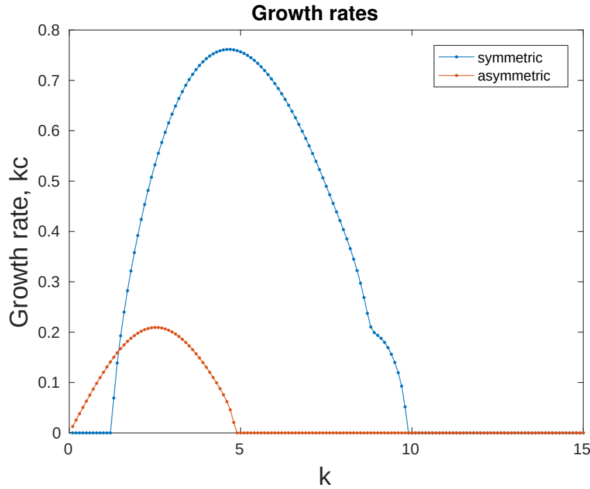
Figure 3.20: The growth rates, kc_i , for symmetric and asymmetric modes, for an eastward sech^2 jet with amplitude U_0 = 1 and a width L = 0.2 .
