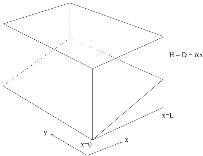
Figure 3.27: A channel with a bottom slope.
