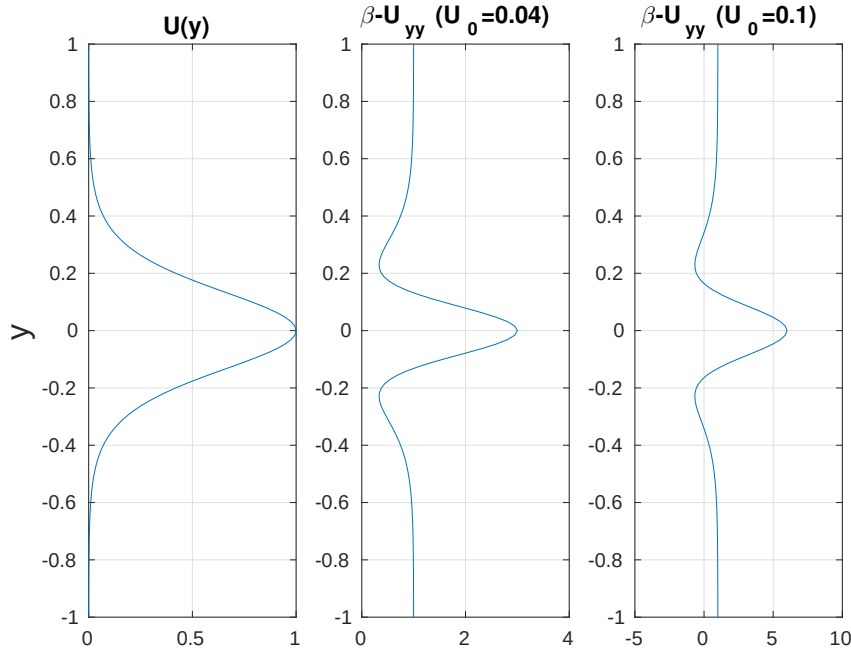
Figure 3.18: An eastward jet (left panel). The middle and right panels show \beta - \frac{\partial^2}{\partial y^2}u for the jet with amplitudes of 0.04 and 0.1, respectively. Only the latter satisfies Rayleigh's criterion for instability.
