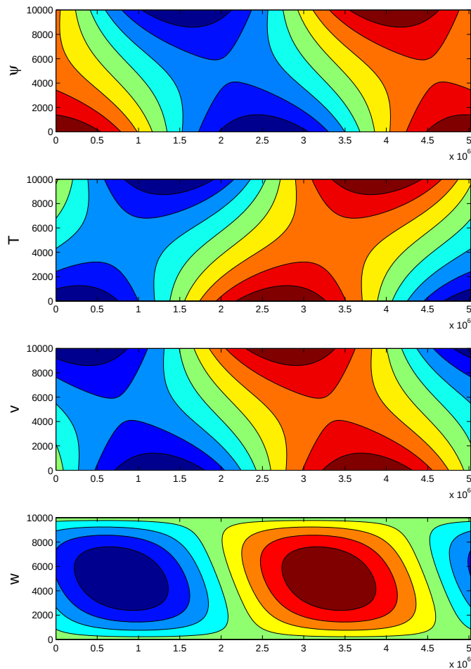
Figure 4.15: The streamfunction (upper), temperature (second), meridional velocity (third) and vertical velocity for the most unstable wave in the Eady problem.
