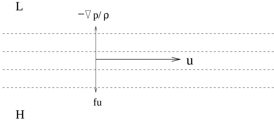
Figure 2.3: The geostrophic balance in the Northern Hemisphere.
