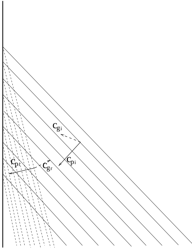
Figure 3.9: A plane Rossby wave reflecting at a western wall. The incident wave is shown by the solid lines and the reflected wave by the dashed lines. The phase velocities are indicated by the solid arrows and the group velocities by the dashed arrows. Note the wavelength in y doesn't change, but the reflected wavelength in x is much shorter. Note too the reflected wave has a phase speed directed toward the wall, but a group velocity away from the wall.
