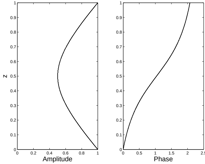
Figure 4.14: The amplitude (left) and phase (right) of the Eady streamfunction vs. height.
