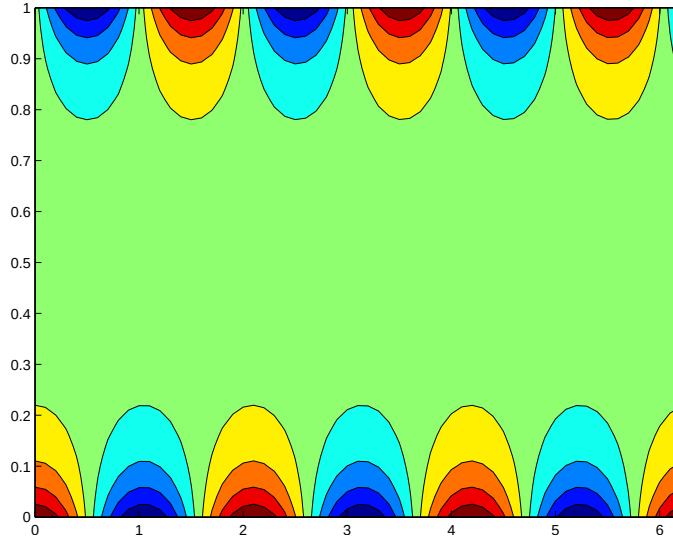
Figure 4.12: The Eady streamfunction in the limit of large \alpha .
