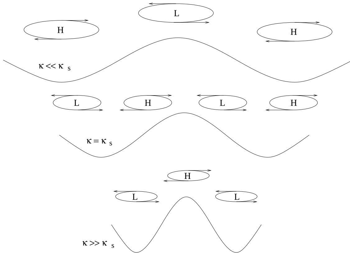
Figure 3.12: The mean pressure distribution over a sinusoidal mountain range. The topographic wavenumber is less than (upper), greater than (bottom) and equal to (middle) the stationary wavenumber.
