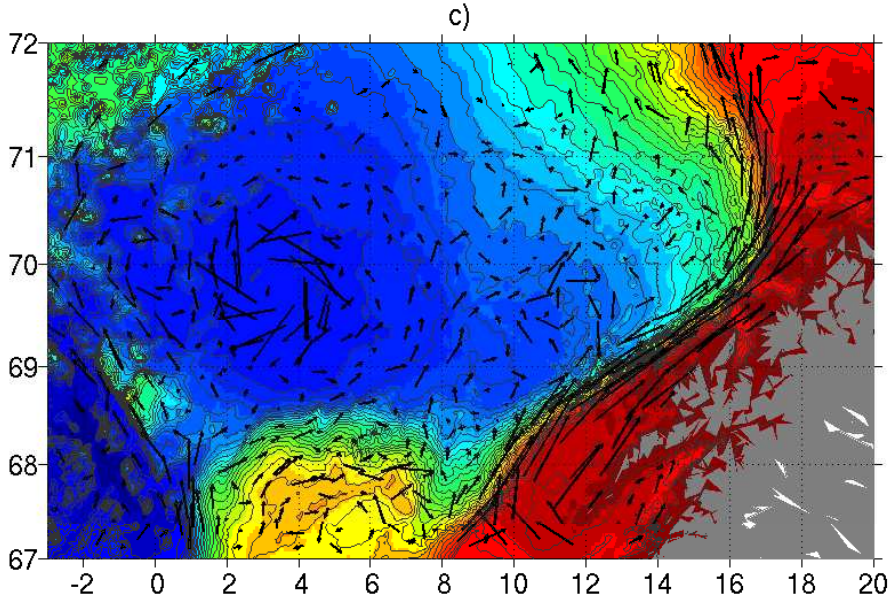
Figure 3.4: Mean velocities estimated from surface drifters in the Lofoten Basin west of Norway. The color contours indicate the water depth. Note the strong flow along the continental margin and the clockwise flow in the center of the basin, near 2° E. From Koszalka et al. (2010).
