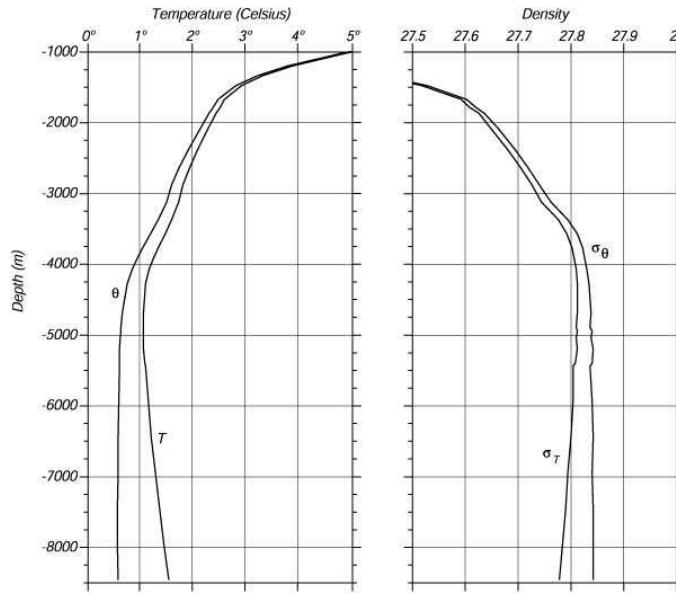
Figure 1.7: The temperature and potential temperature (left panel) and the potential density, \sigma_\theta (right panel), plotted vs. depth. The additional density, \sigma_T , is an alternate form of the potential density. The data come from the Kermadec trench in the Pacific and are described by Warren (1973). Courtesy of Ocean World at Texas A&M University.
