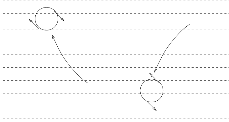
Figure 3.1: The change in relative vorticity due to northward or southward motion relative to \beta y .
