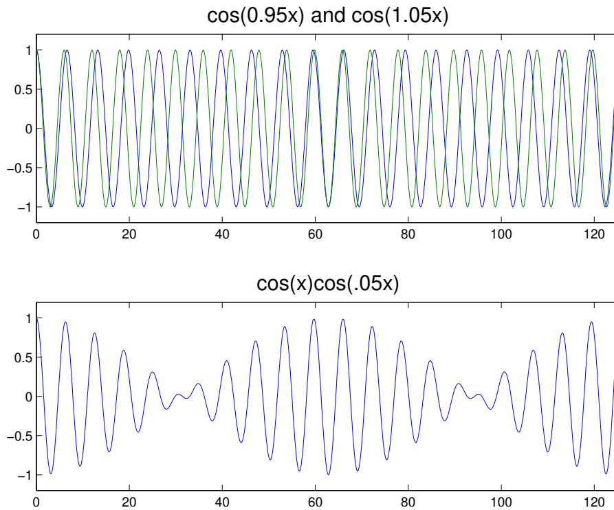
Figure 3.8: Two waves with nearly the same wavelength (upper panel) and their sum (lower panel).
