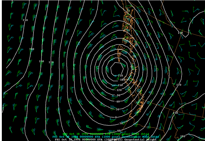
Figure 2.5: A low pressure system off the west coast of the United States. The green vectors are observed winds and the blue are geostrophic. Courtesy of the University of Washington.
