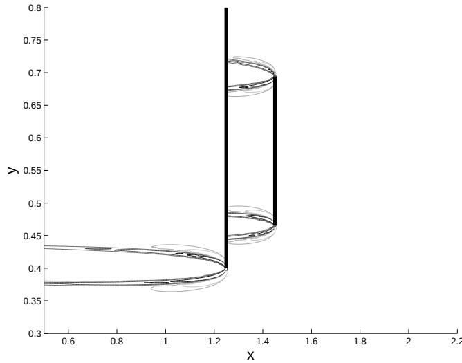
Figure 3.25: The PV gradient for the solution in Fig. (3.24). The gradient changes sign rapidly in the three jet regions. From LaCasce and Isachsen (2007).
