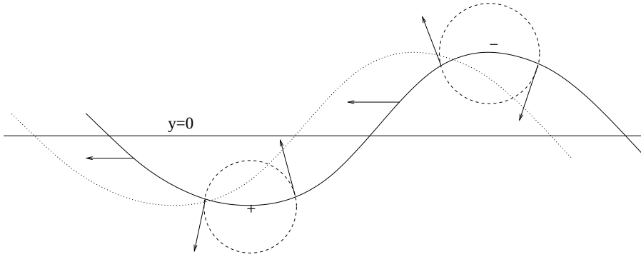
Figure 3.5: Relative vorticity induced in a Rossby wave. Fluid advected northwards acquires negative vorticity and fluid advected southwards positive vorticity.
