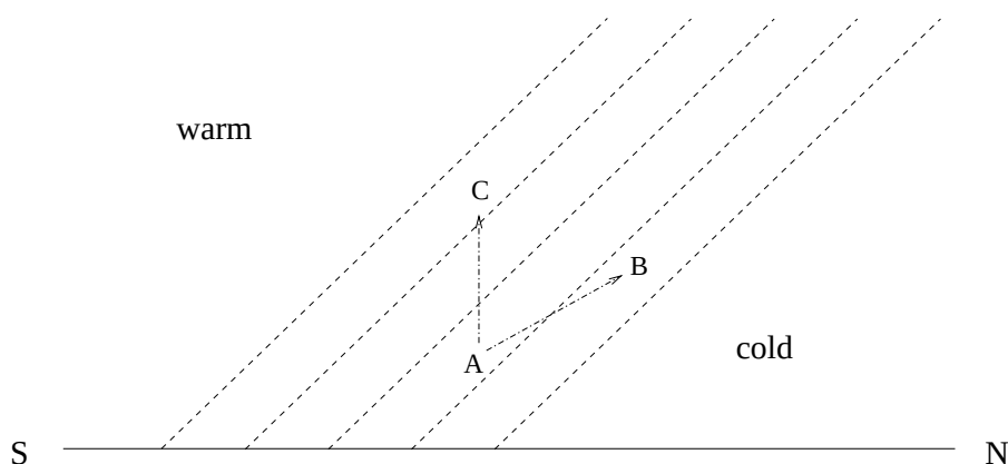
Figure 4.9: Slantwise convection. The slanted isotherms are accompanied by a thermal wind shear. The parcel A is colder, and thus heavier, than parcel C, implying static stability. But A is lighter than B. So A and B can be interchanged, releasing potential energy.
