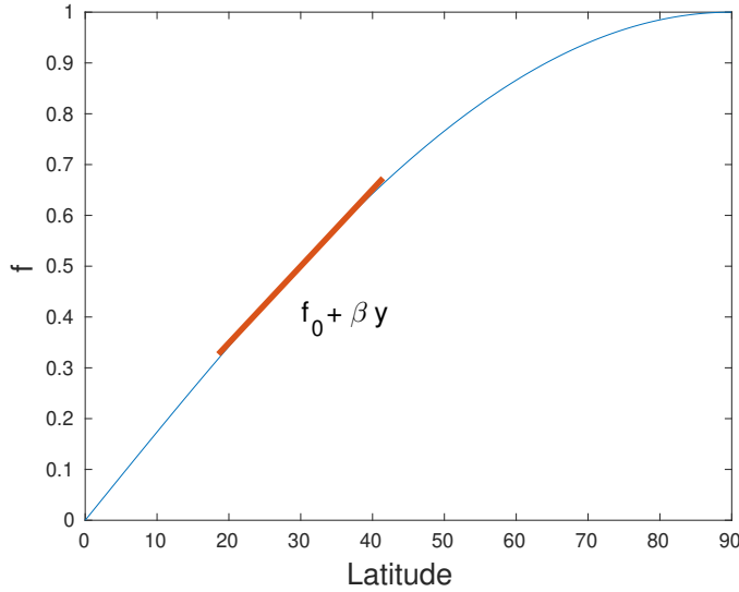
Figure 2.10: The Coriolis parameter, as a function of latitude, and the \beta -plane approximation with a central latitude of \theta = 30^\circ .
