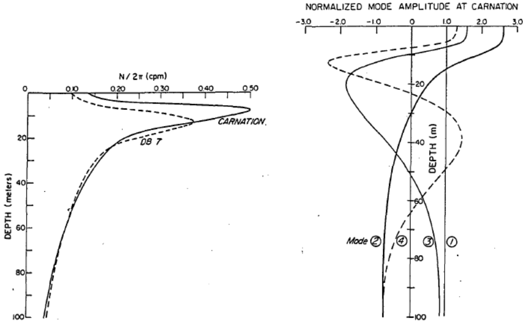
Figure 4.4: The buoyancy frequency (left panel) and the corresponding vertical modes (right panel) from a location on the continental shelf off Oregon. From Kundu et al. (1974).
