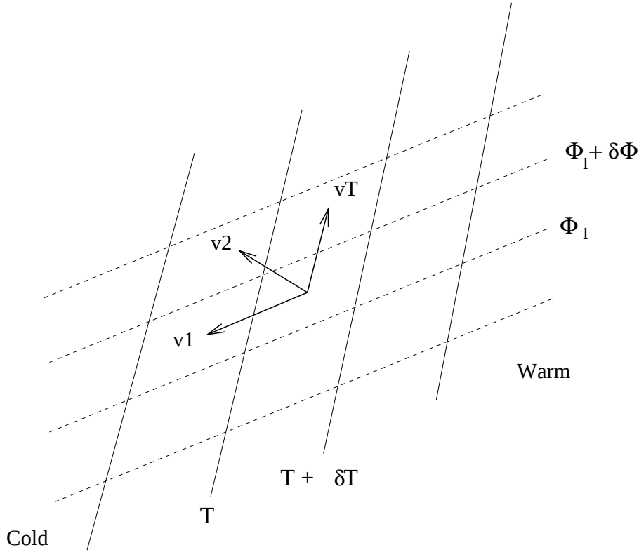
Figure 2.15: Thermal wind between two layers (1 and 2). The geopotential height contours for the lower layer, \Phi_1 , are the dashed lines and the temperature contours are the solid lines.
