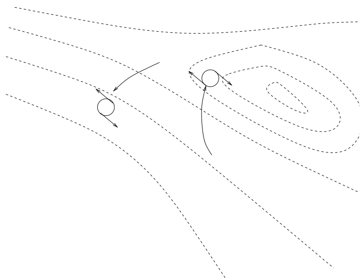
Figure 3.2: The change in relative vorticity due to motion across geostrophic contours with topography.
