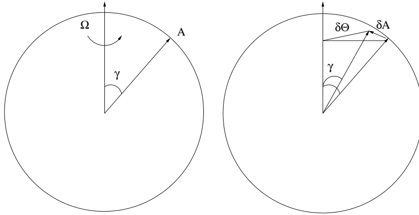
Figure 1.3: The effect of rotation on a vector, A , which is otherwise stationary. The vector rotates through an angle, \delta\Theta , in a time \delta t .
