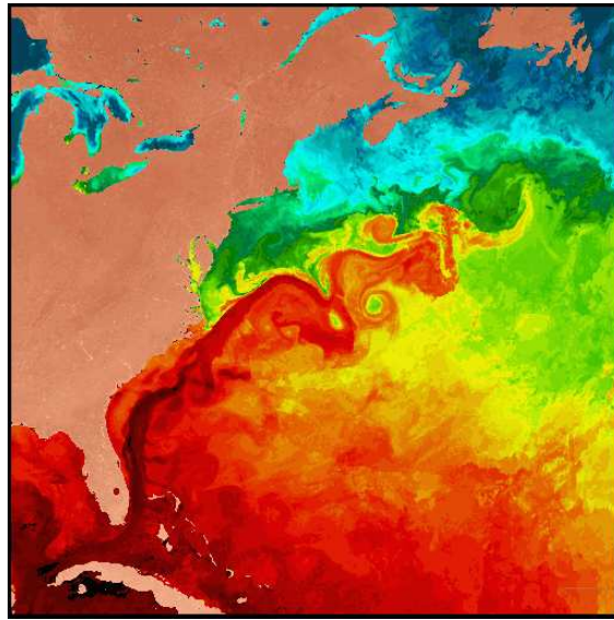
Figure 2.12: The sea surface temperature in the North Atlantic. The Gulf Stream lies between the warm Sargasso Sea and the cold waters to the north.
