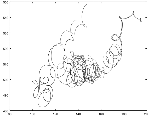
Figure 2.7: A pair of drifting buoys on the surface in the Gulf of Mexico, deployed as part of the GLAD experiment. The pair were deployed in the upper right corner of the figure. Courtesy of the University of Miami.
