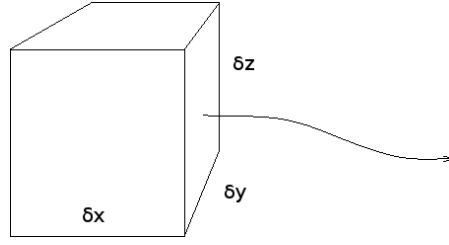
Figure 1.1: A infinitesimal element of fluid, with volume \delta V , moving with the flow.
