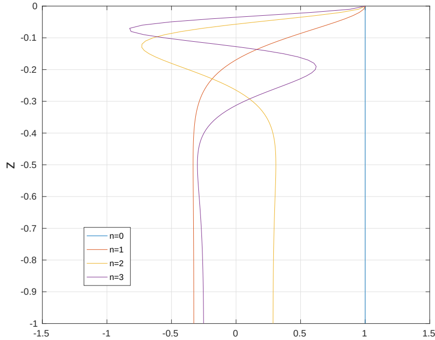
Figure 4.3: The baroclinic modes with exponential stratification. The e-folding rate for the stratification, \alpha , is 2.5.
