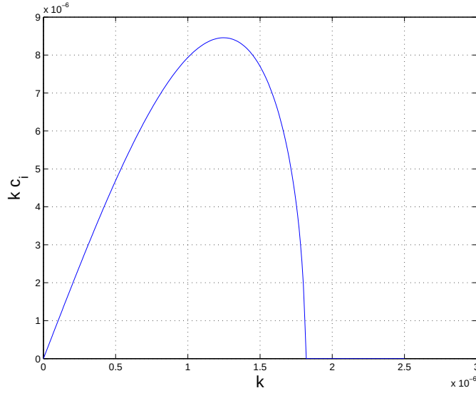
Figure 4.13: The Eady growth rate as a function of the wavenumber, k .
