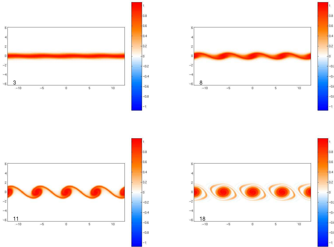
Figure 3.22: Barotropic instability of a jet with a Gaussian profile in relative vorticity. Courtesy of G. Hakim, Univ. of Washington.
