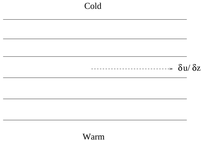
Figure 2.14: The thermal wind shear associated with a temperature gradient in the y -direction.
