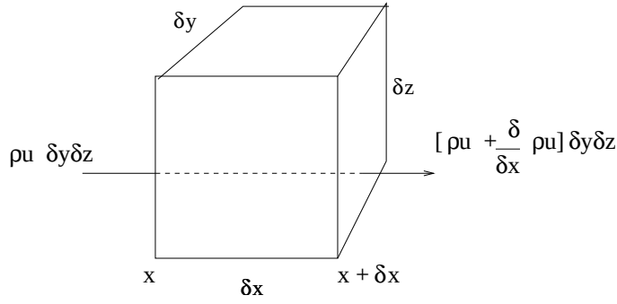
Figure 1.2: A infinitesimal element of fluid, with volume \delta V , fixed in space and with fluid flowing through it.
