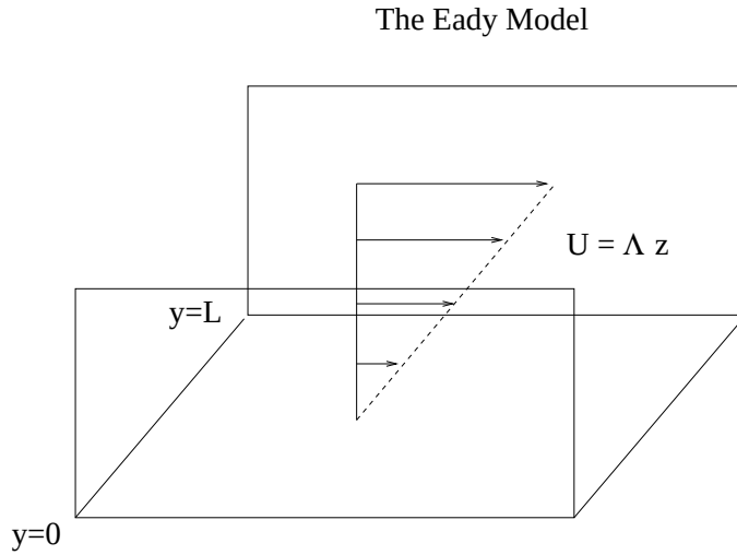
Figure 4.10: The configuration for the Eady model.
