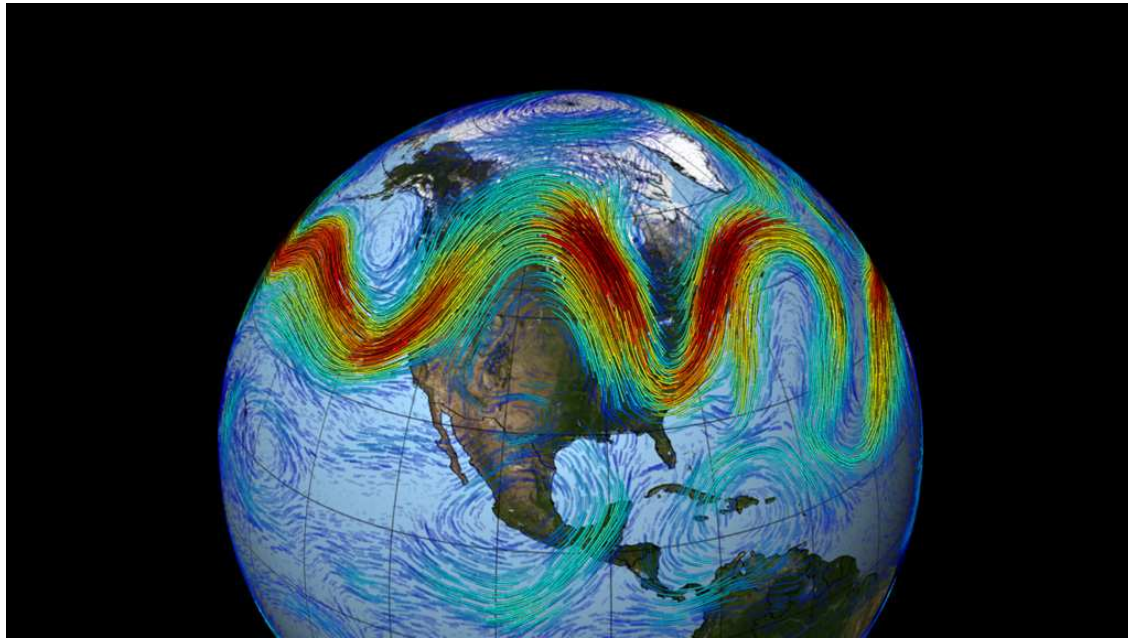
Figure 3.6: An example of Rossby waves in the atmosphere. The Jet Stream, flowing eastward, is superimposed over westward-propagating Rossby waves. Courtesy of NASA.
