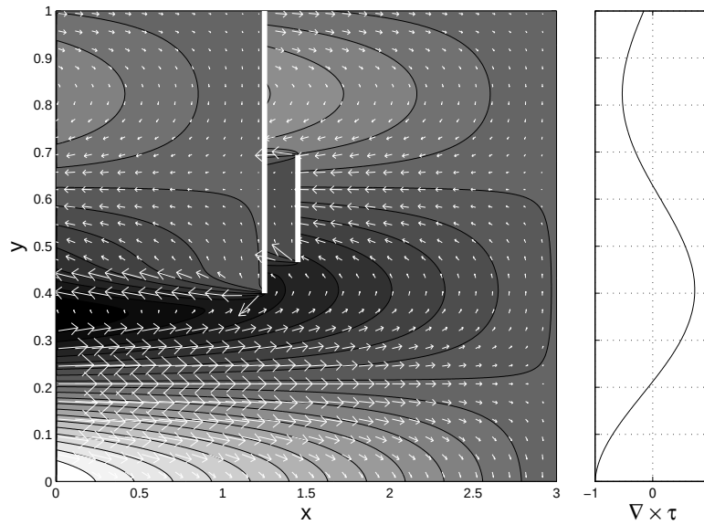
Figure 3.24: A Stommel-like solution for the Indian Ocean. The curl of the wind stress is indicated in the right panel. From LaCasce and Isachsen (2007).
