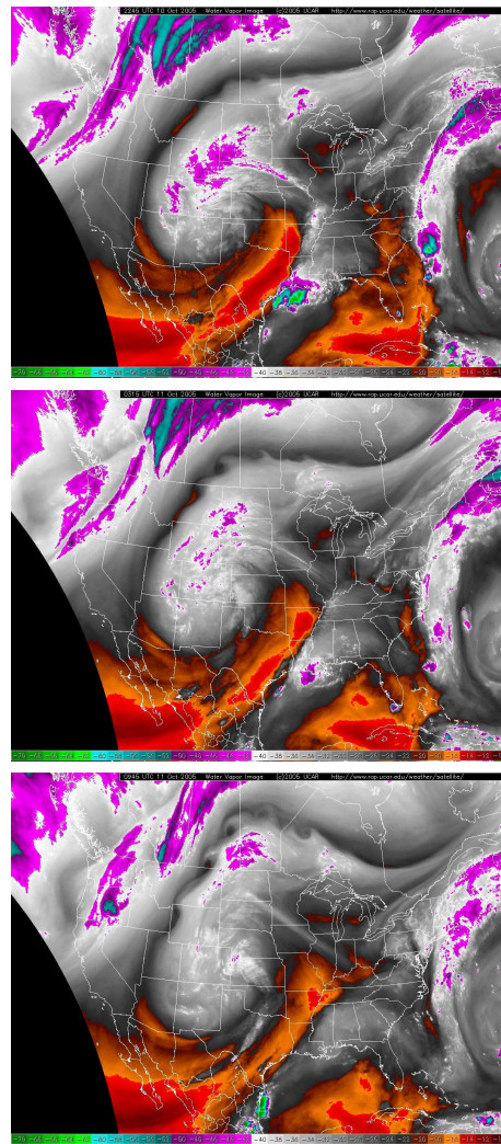
Figure 3.23: Barotropic instability of a filament of dry air, observed from water vapor infrared satellite imagery. The images were taken on the 11th of October, 2005, at 22:45 pm, 3:15 am and 9:45 am, respectively. Courtesy of G. Hakim, Univ. of Washington.
