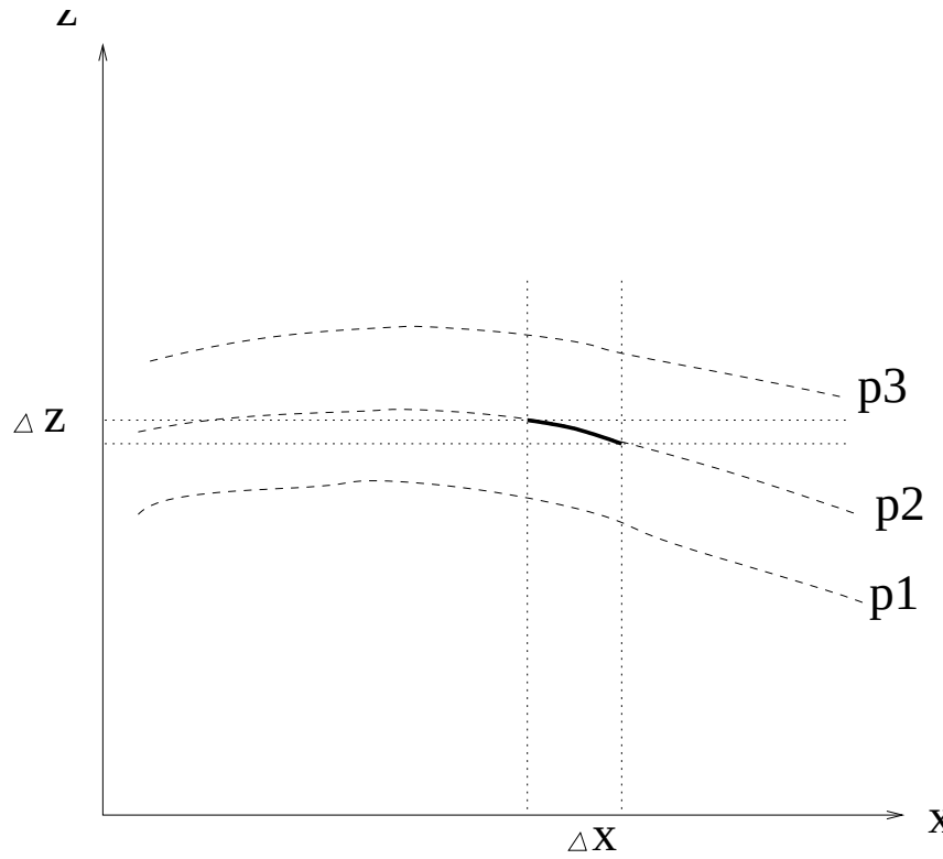
Figure 2.11: Pressure surfaces in (x, z) .
