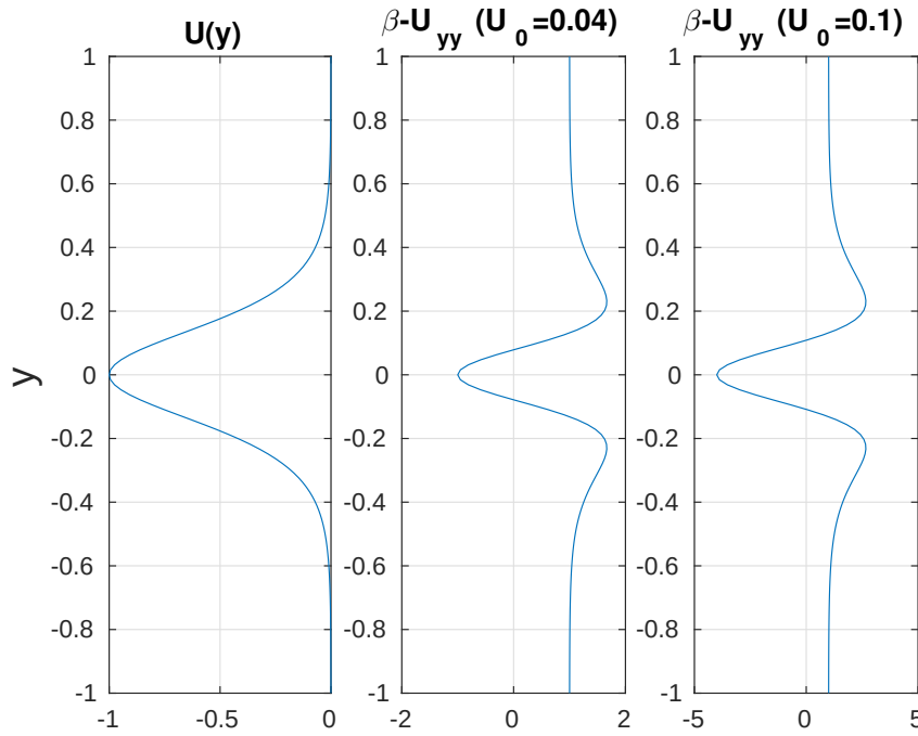
Figure 3.19: A westward jet (left panel). The middle and right panels again show \beta - \frac{\partial^2}{\partial y^2} u for the jet, with amplitudes of 0.04 and 0.1. Note that both satisfy Rayleigh's criterion for instability.
