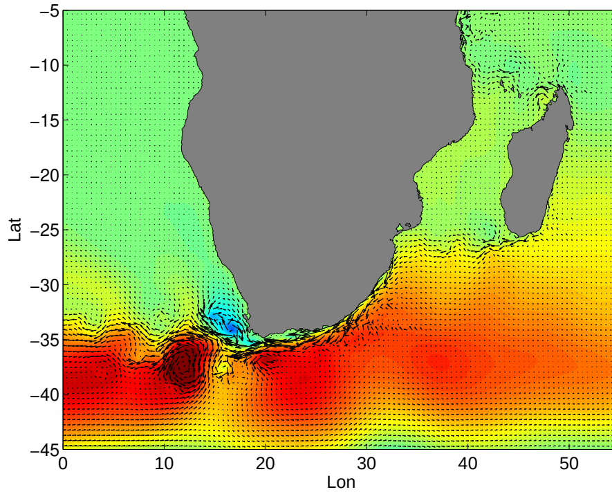
Figure 3.26: The sea surface height from a barotropic numerical simulation of the southern Indian and Atlantic Oceans. From LaCasce and Isachsen (2007).
