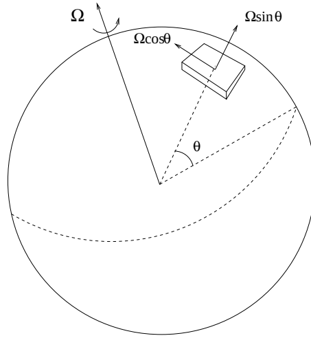
Figure 1.5: We examine the dynamics of a rectangular region of ocean or atmosphere centered at latitude \theta .
