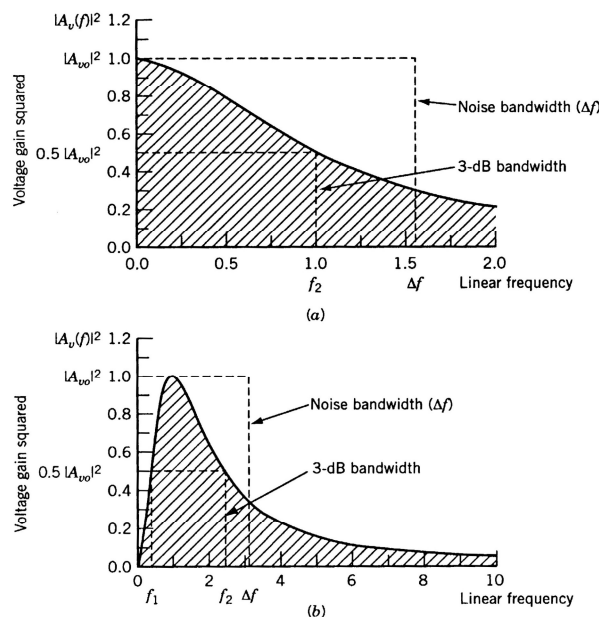
Figure 1-3 Definition of noise bandwidth.
