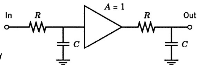
Figure 1-4 Cascaded low-pass filter.
