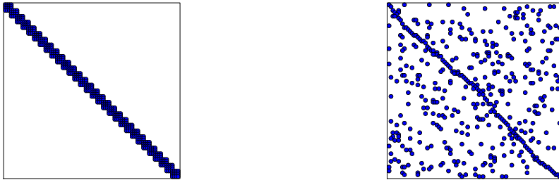
Fig. 4.21 Matrix sparsity pattern for left-to-right numbering (left) and random numbering (right) of nodes in P3 elements.
