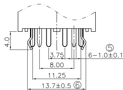
TERMINAL DETAIL (2:1)
