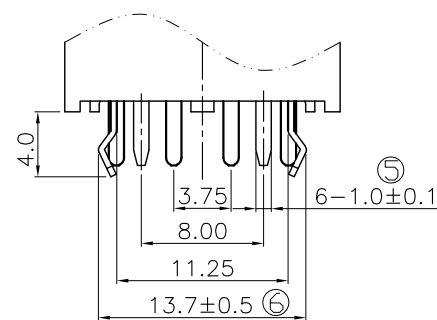
TERMINAL DETAIL (2:1)
