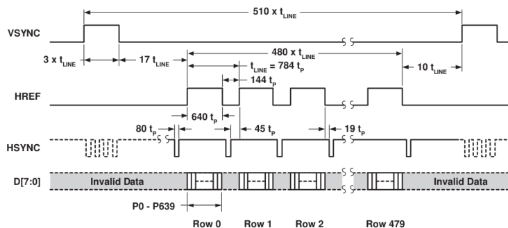
Fig. 5. Readout timing diagram for a "VGA" (640 x 480)
