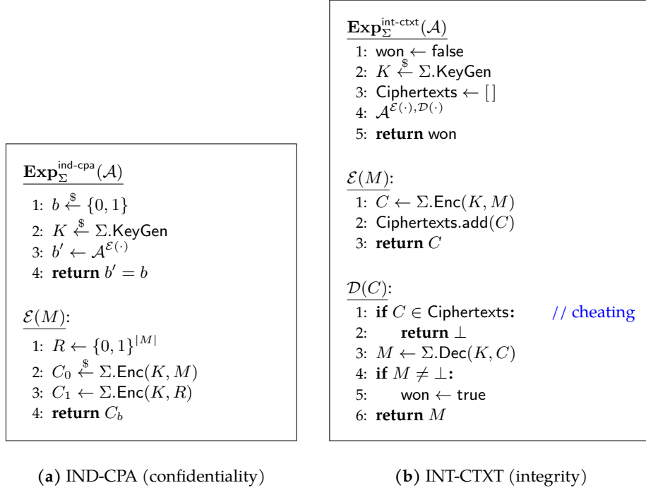
Figure 1: Separate confidentiality and integrity security experiments for an authenticated encryption scheme \Sigma .
