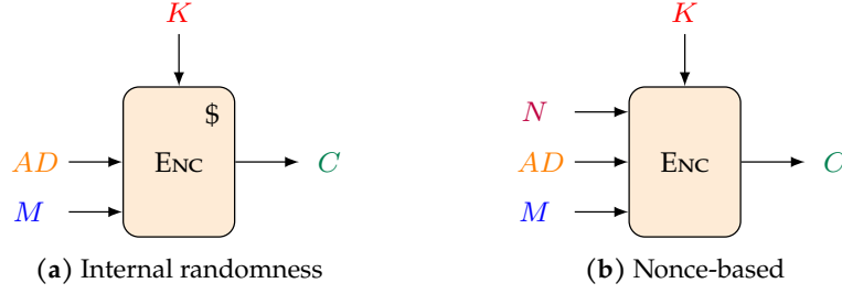
Figure 4: AEAD
