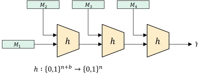
Figure 1: Simplified Merkle-Damgård using no IV and no encoding of the message length in the final padding block. Here |M_1| = n and |M_2| = |M_3| = |M_4| = b .
