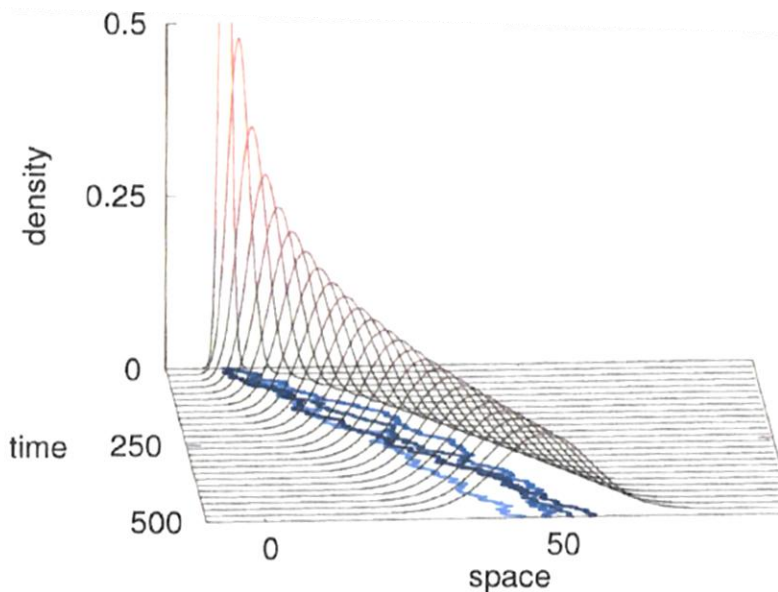
Fig. 5.9 Evolution of a probability density modeled by the Fokker-Planck equation, Eq. (5.25). Example in 1-d space with a drift of A = 0.1 and diffusion B = 0.3 . Shown is the probability density and four example realizations of the corresponding Langevin equation
