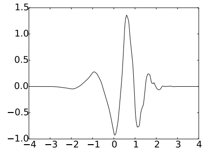
(f) \psi for N=4
