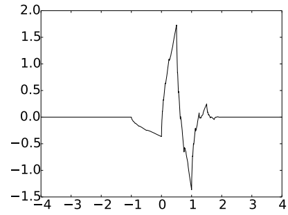
(b) \psi for N=2
