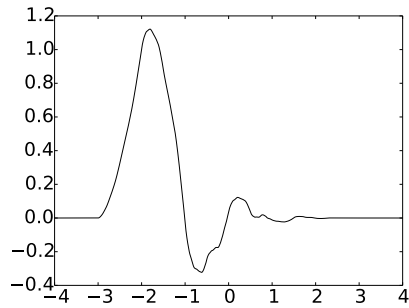
(e) \phi for N=4
