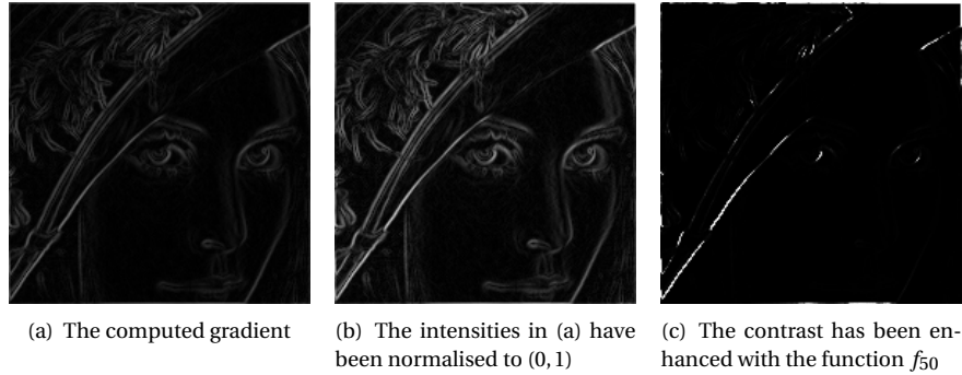
Figure 9.11: Computing the gradient.
