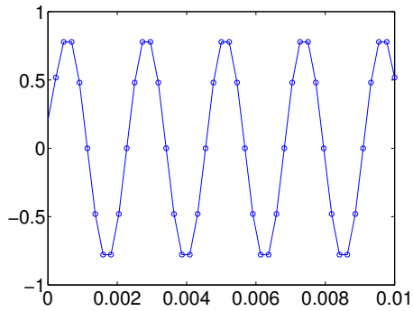
(b) The result of applying the filter from row 4 of Pascal's triangle
