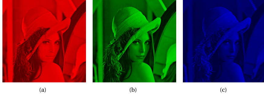
Figure 9.3: The red (a), green (b), and blue (c) components of the colour image in Figure 9.1.
