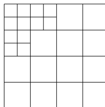
Figure 10.19: The fingerprint image after several DWT's
