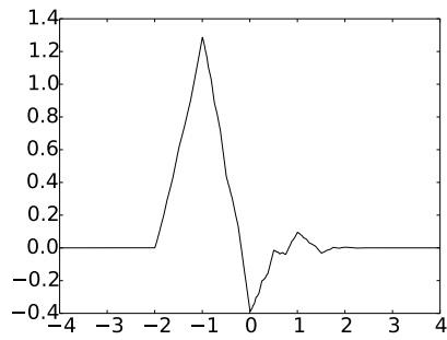
(c) \phi for N=3
