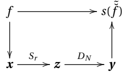
Figure 4.3: The connections between the new mapping S_r , sampling, and interpolation. The right vertical arrow represents interpolation with the DCT, i.e. that we compute \sum_{n=0}^{N-1} y_n d_{n,N} \cos(2\pi(n/2)t/T) for values of t .
