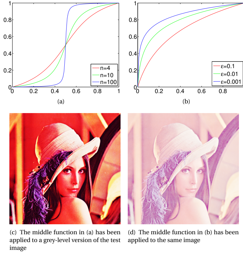
Figure 9.6: The plots in (a) and (b) show some functions that can be used to improve the contrast of an image.
