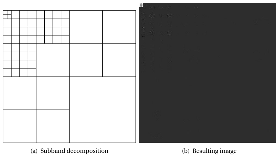
Figure 10.20: The wavelet subband decomposition with the resulting image, as employed by the FBI
