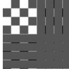
Figure 10.6: The chess pattern example image after application of the DWT2. The Haar wavelet was used.
