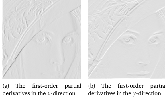
Figure 9.12: In both images, the computed numbers have been normalised and the contrast enhanced.
