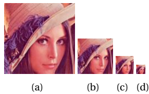
Figure 10.7: The corresponding thumbnail images for the Image of Lena, obtained with a DWT of 1, 2, 3, and 4 levels.
