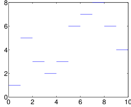
Figure 5.2: A piecewise constant function.
