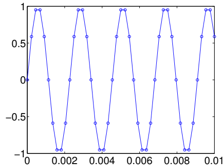
(a) The original sound signal
