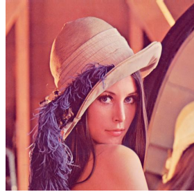
(a) The image unaltered
