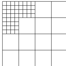
Figure 10.20: The wavelet subband decomposition with the resulting image, as employed by the FBI
