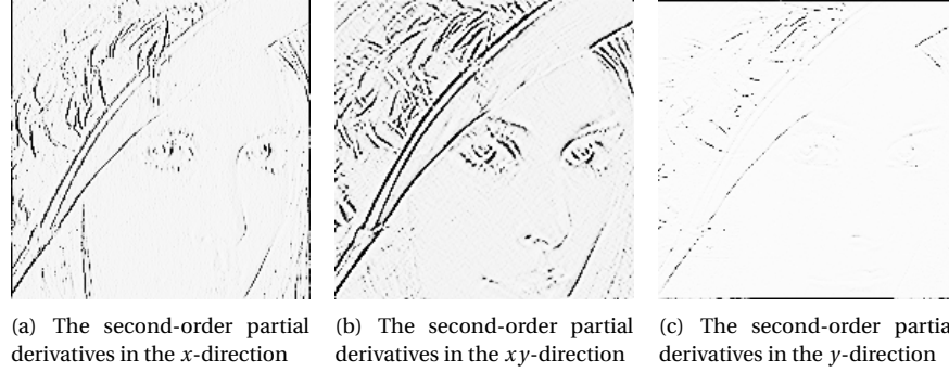
Figure 9.13: In all images, the computed numbers have been normalised and the contrast enhanced.
