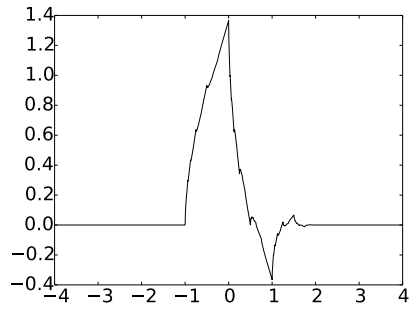
(a) \phi for N=2
