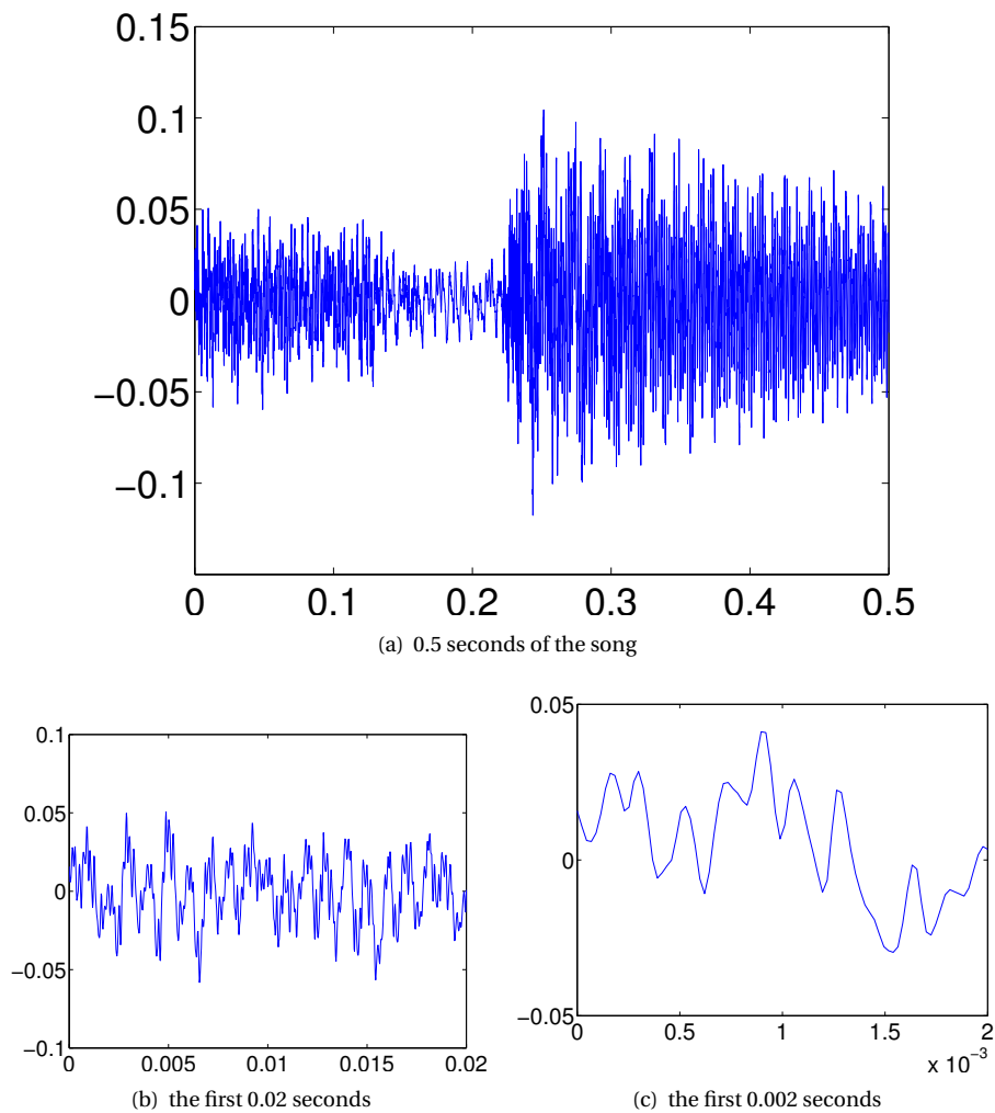
Figure 1.2: Variations in air pressure during parts of a song.
