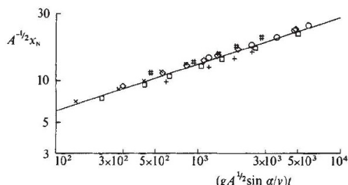
Fig. 3 The length of the two-dimensional flow, normalized with respect to A^{1/2} , as a function of a suitably non-dimensional time. The straight line is the theoretical prediction obtained from equation (7). The experimental points are for values of \nu , \sin \alpha , A in cgs units of: \square , 12.9, 0.093, 8.9; \diamond , 12.9, 0.20, 3.1; \circ , 12.9, 0.65, 5.9; + , 9.8, 0.20, 9.0; \times , 9.8, 0.15, 3.6; \# , 1.2, 0.11, 1.0.
