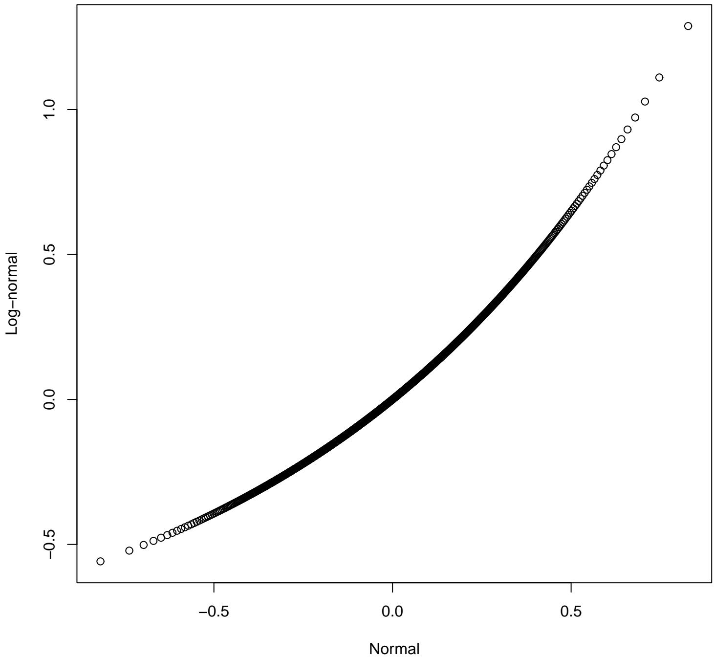
Log-normal equity against normal
