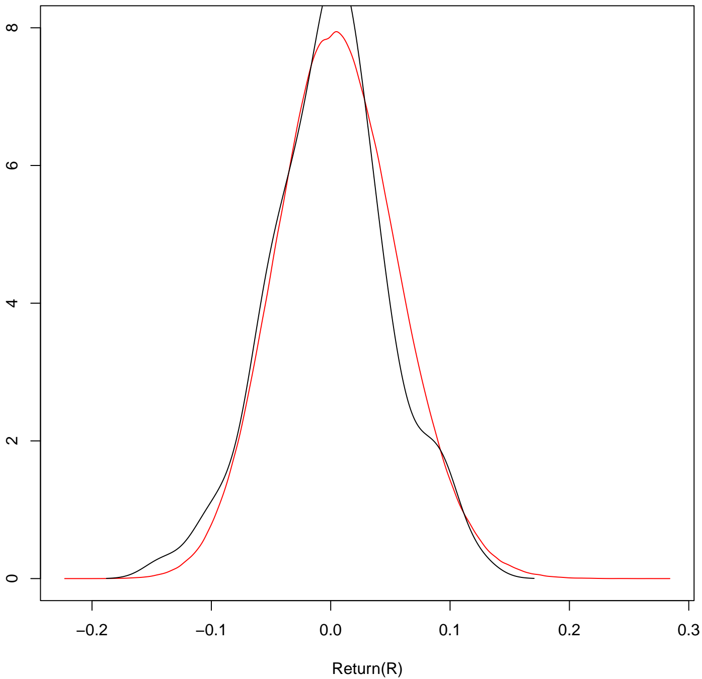
Density estimation with 100 observations
