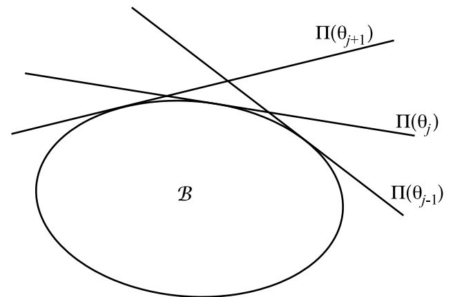
Fig. 4.4. Ideal case: All hyperplanes support B .
