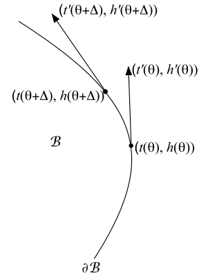
Fig. 3.2. Derivatives.
