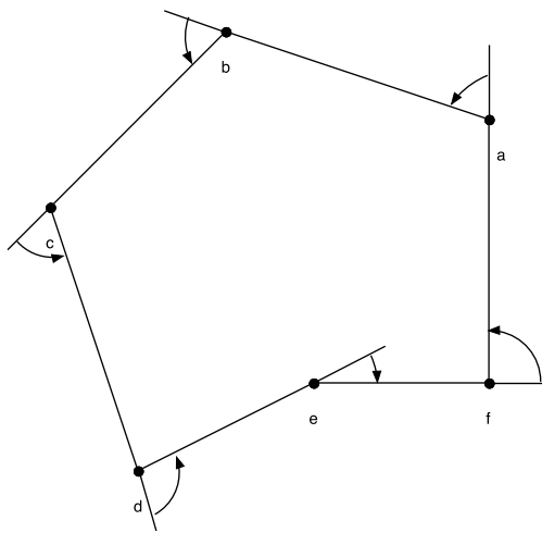
Fig. 5.2. Measuring polygon angles.
