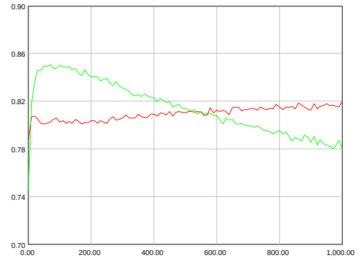
Fig. 5. I_{NB}^{(1)}(t) (red) and I_{NB}^{(2)}(t) (green) - Local time model
