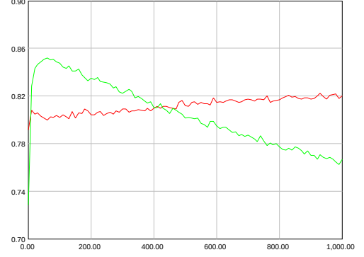
Fig. 4. I_{NB}^{(1)}(t) (red) and I_{NB}^{(2)}(t) (green) - Global time model
