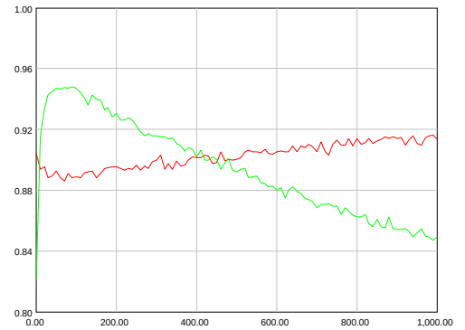
Fig. 6. I_{NB}^{*(1)}(t) (red) and I_{NB}^{*(2)}(t) (green) - Global time model
