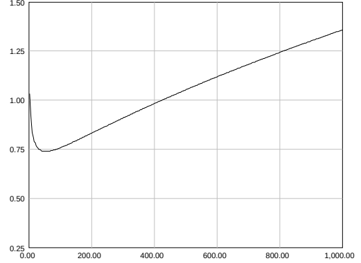
Fig. 1. The intensity function \lambda_2^{(1)}(t)
