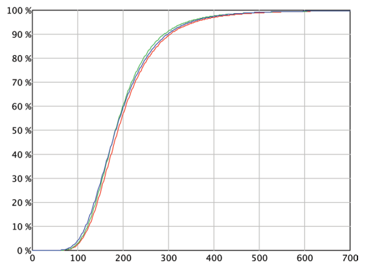
Figure 1. Estimated cumulative distributions for the accumulated consequences using the no overlap model (red curve), full overlap model (green curve) and the partial overlap model (blue curve), \beta_R = 0.2 .
