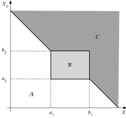
Fig. 1. The sets \mathcal{A} , \mathcal{B} and \mathcal{C} .
