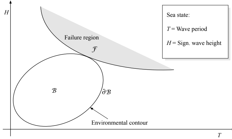
Figure 1: An environmental contour and a potential failure region
