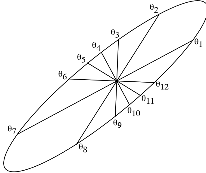
Figure 2: Evenly spaced \theta_1, \dots, \theta_n
